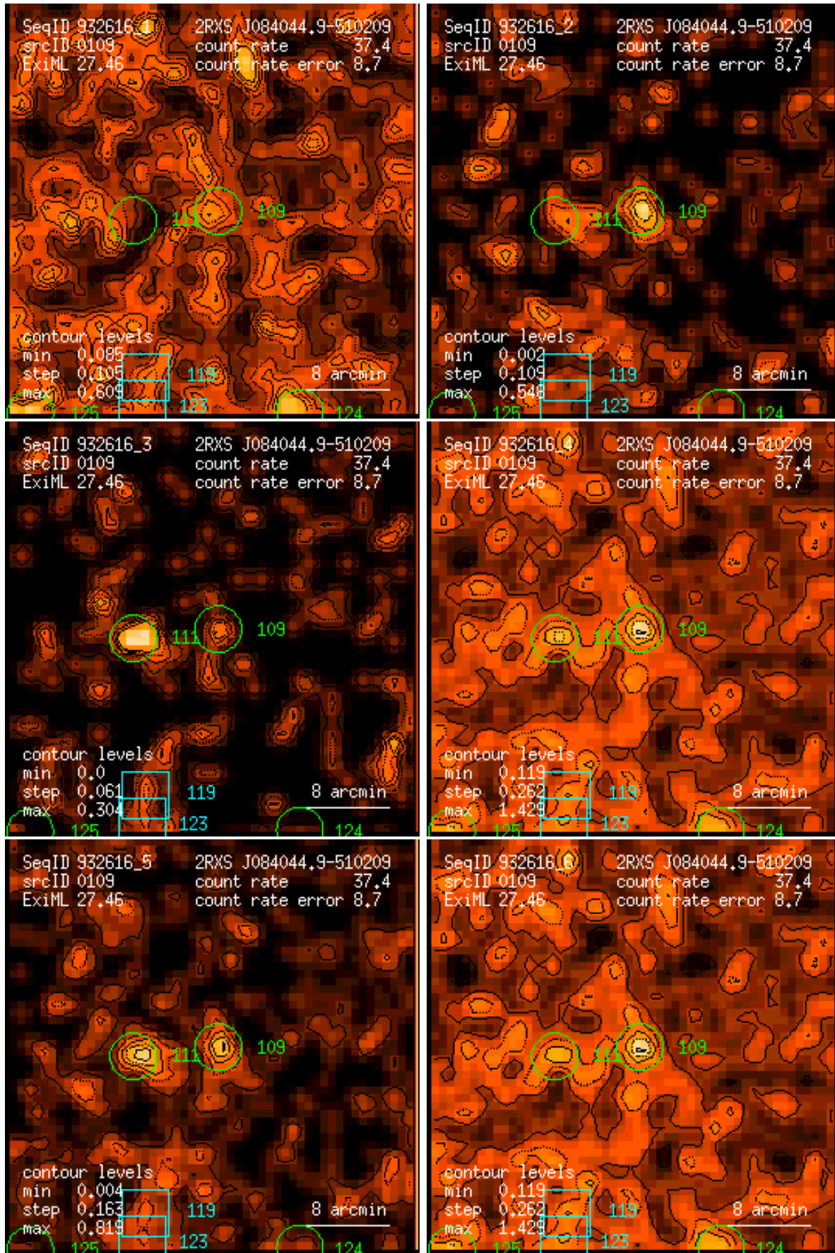
Figure 109: RASS 932616: detection 0109: band rate images, Gaussian filter: (1) PSPC channels 11 – 41, (2) 52 – 90, (3) 91 – 201, (4) 11 – 235, (5) 52 – 201, (6) 11 – 201. Broad band rates in counts/ks. Band rate contour levels in counts/ks/arcmin 2 .
