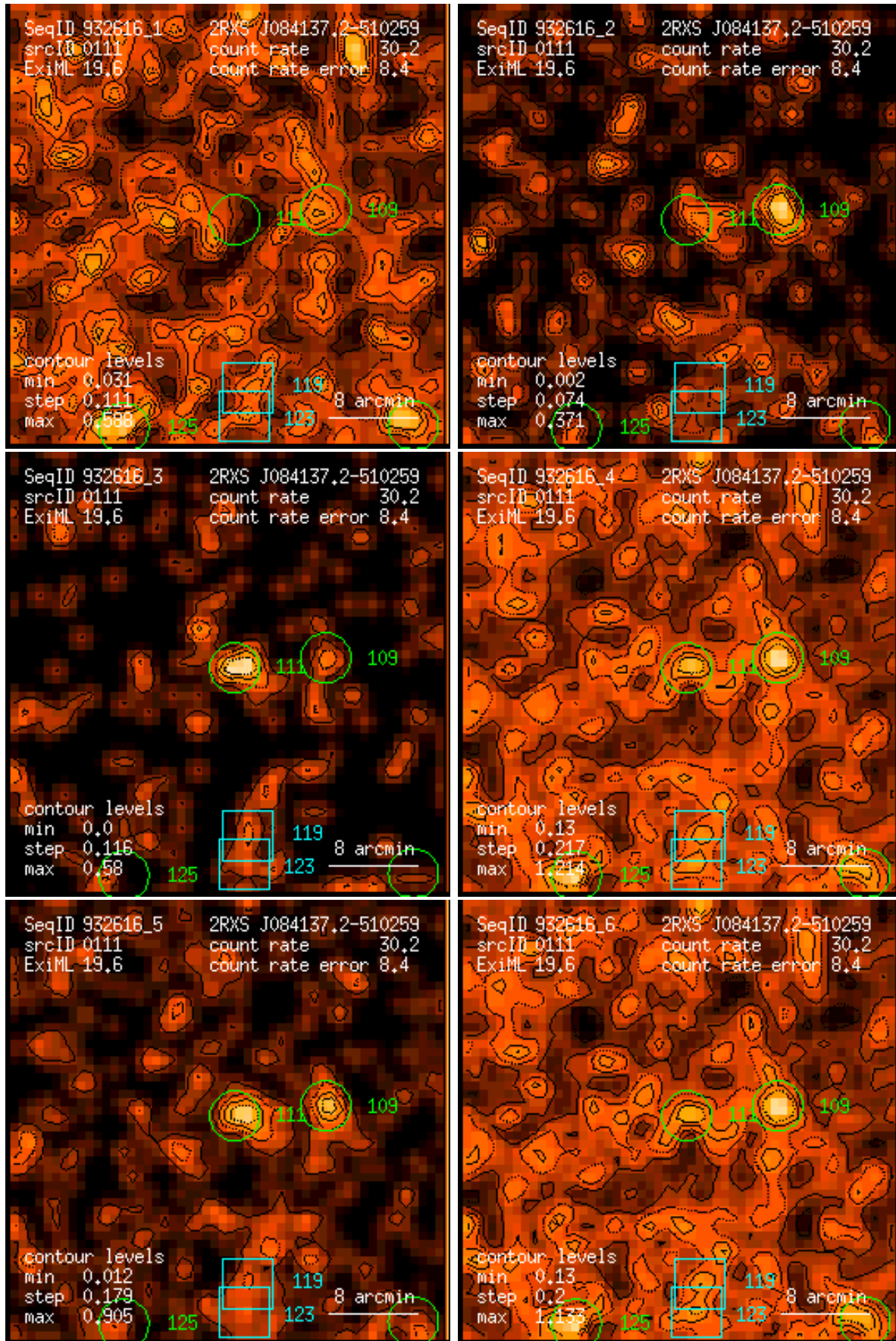
Figure 111: RASS 932616: detection 0111: band rate images, Gaussian filter: (1) PSPC channels 11 – 41, (2) 52 – 90, (3) 91 – 201, (4) 11 – 235, (5) 52 – 201, (6) 11 – 201. Broad band rates in counts/ks. Band rate contour levels in counts/ks/arcmin 2 .
