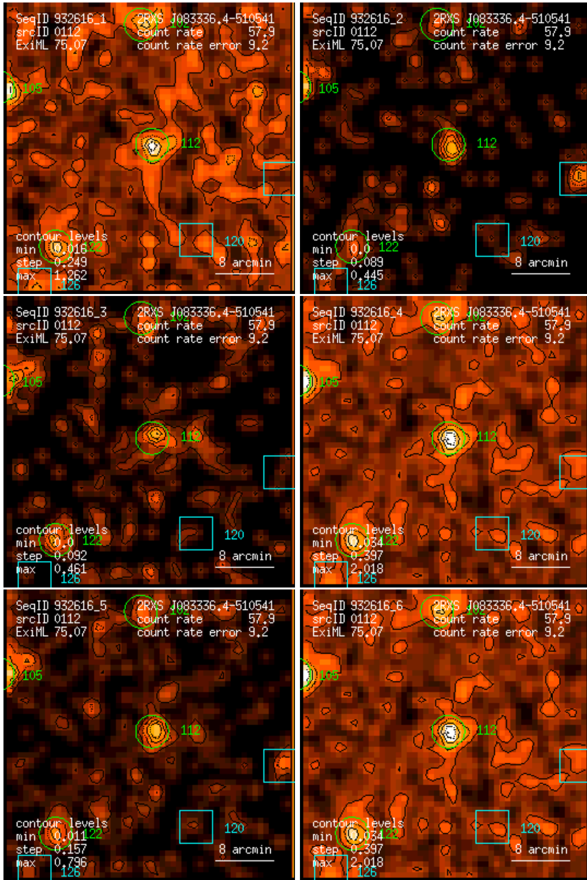
Figure 112: RASS 932616: detection 0112: band rate images, Gaussian filter: (1) PSPC channels 11 – 41, (2) 52 – 90, (3) 91 – 201, (4) 11 – 235, (5) 52 – 201, (6) 11 – 201. Broad band rates in counts/ks. Band rate contour levels in counts/ks/arcmin 2 .
