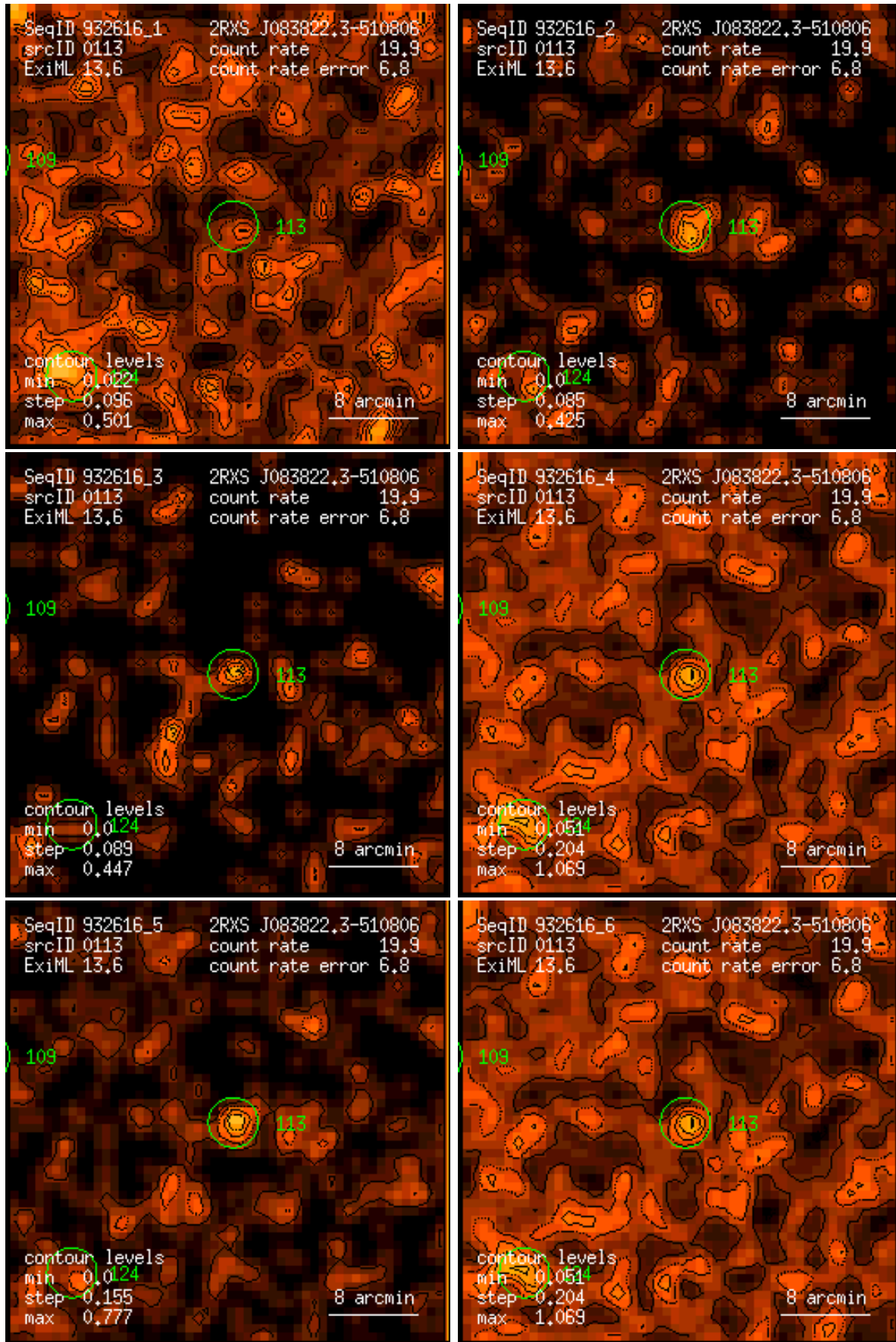
Figure 113: RASS 932616: detection 0113: band rate images, Gaussian filter: (1) PSPC channels 11 – 41, (2) 52 – 90, (3) 91 – 201, (4) 11 – 235, (5) 52 – 201, (6) 11 – 201. Broad band rates in counts/ks. Band rate contour levels in counts/ks/arcmin 2 .
