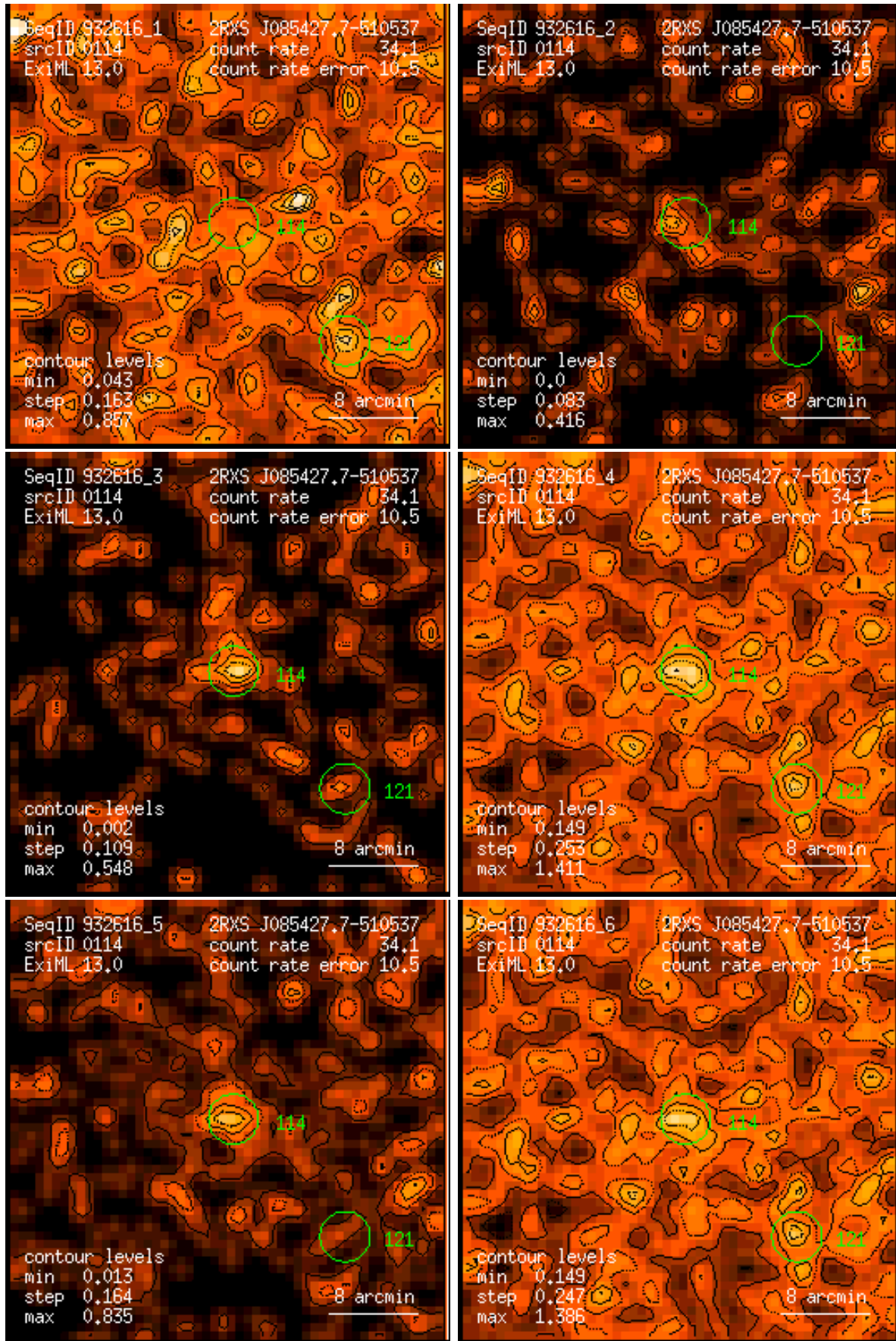
Figure 114: RASS 932616: detection 0114: band rate images, Gaussian filter: (1) PSPC channels 11 – 41, (2) 52 – 90, (3) 91 – 201, (4) 11 – 235, (5) 52 – 201, (6) 11 – 201. Broad band rates in counts/ks. Band rate contour levels in counts/ks/arcmin 2 .
