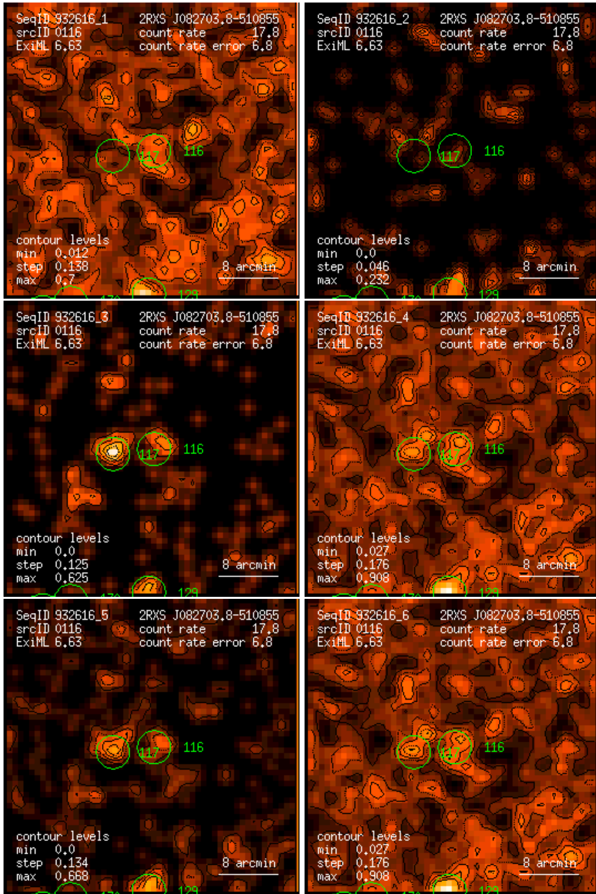
Figure 116: RASS 932616: detection 0116: band rate images, Gaussian filter: (1) PSPC channels 11 – 41, (2) 52 – 90, (3) 91 – 201, (4) 11 – 235, (5) 52 – 201, (6) 11 – 201. Broad band rates in counts/ks. Band rate contour levels in counts/ks/arcmin 2 .
