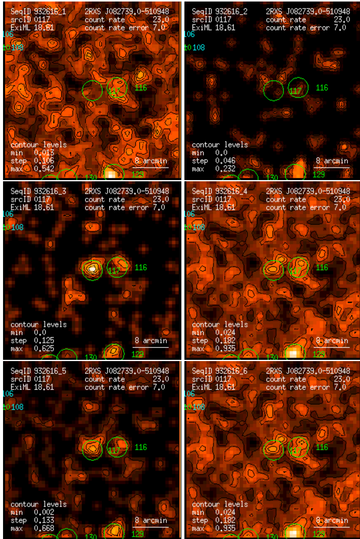
Figure 117: RASS 932616: detection 0117: band rate images, Gaussian filter: (1) PSPC channels 11 – 41, (2) 52 – 90, (3) 91 – 201, (4) 11 – 235, (5) 52 – 201, (6) 11 – 201. Broad band rates in counts/ks. Band rate contour levels in counts/ks/arcmin 2 .
