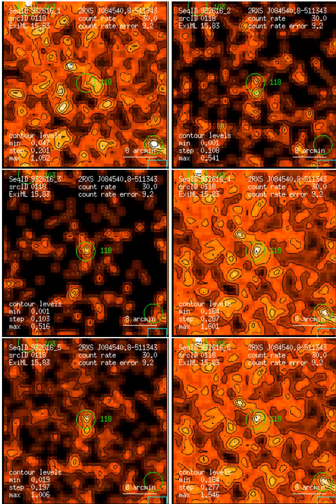
Figure 118: RASS 932616: detection 0118: band rate images, Gaussian filter: (1) PSPC channels 11 – 41, (2) 52 – 90, (3) 91 – 201, (4) 11 – 235, (5) 52 – 201, (6) 11 – 201. Broad band rates in counts/ks. Band rate contour levels in counts/ks/arcmin 2 .
