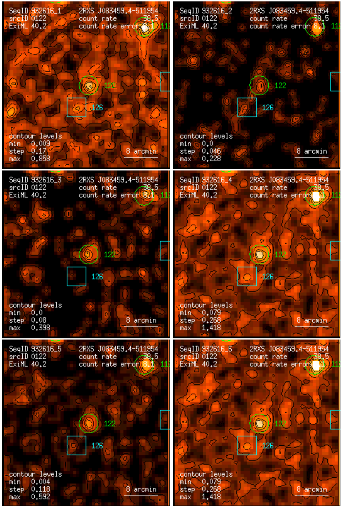
Figure 122: RASS 932616: detection 0122: band rate images, Gaussian filter: (1) PSPC channels 11 – 41, (2) 52 – 90, (3) 91 – 201, (4) 11 – 235, (5) 52 – 201, (6) 11 – 201. Broad band rates in counts/ks. Band rate contour levels in counts/ks/arcmin 2 .
