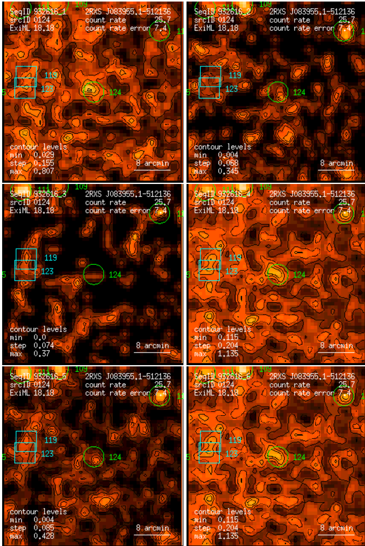
Figure 124: RASS 932616: detection 0124: band rate images, Gaussian filter: (1) PSPC channels 11 – 41, (2) 52 – 90, (3) 91 – 201, (4) 11 – 235, (5) 52 – 201, (6) 11 – 201. Broad band rates in counts/ks. Band rate contour levels in counts/ks/arcmin 2 .
