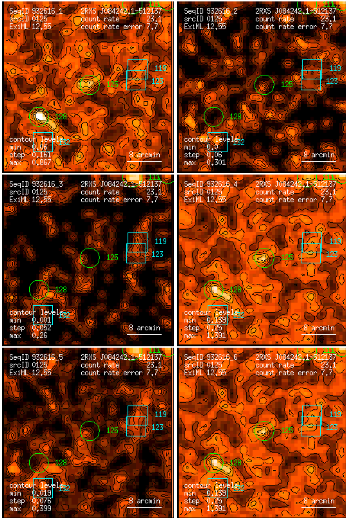
Figure 125: RASS 932616: detection 0125: band rate images, Gaussian filter: (1) PSPC channels 11 – 41, (2) 52 – 90, (3) 91 – 201, (4) 11 – 235, (5) 52 – 201, (6) 11 – 201. Broad band rates in counts/ks. Band rate contour levels in counts/ks/arcmin 2 .
