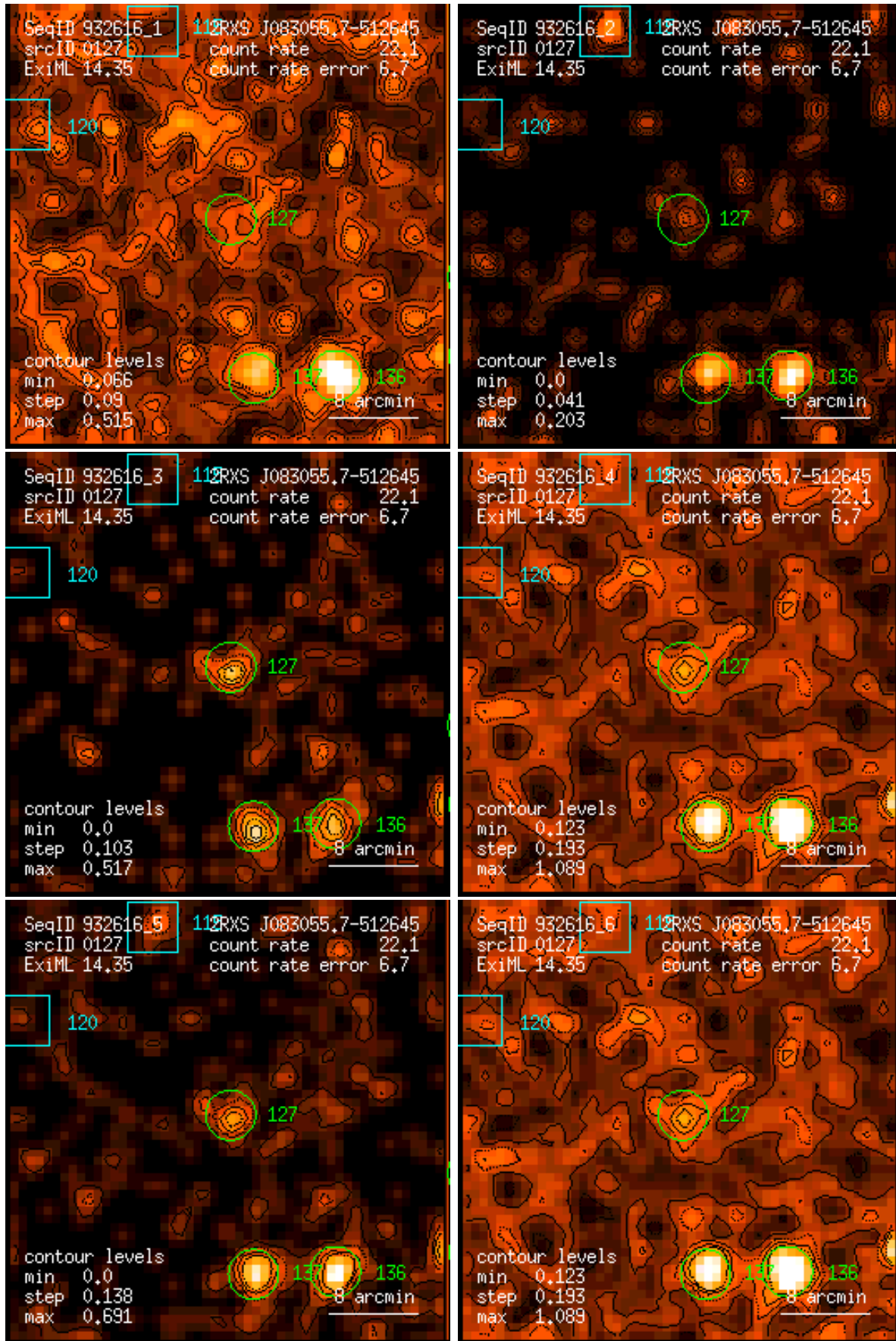
Figure 127: RASS 932616: detection 0127: band rate images, Gaussian filter: (1) PSPC channels 11 – 41, (2) 52 – 90, (3) 91 – 201, (4) 11 – 235, (5) 52 – 201, (6) 11 – 201. Broad band rates in counts/ks. Band rate contour levels in counts/ks/arcmin 2 .
