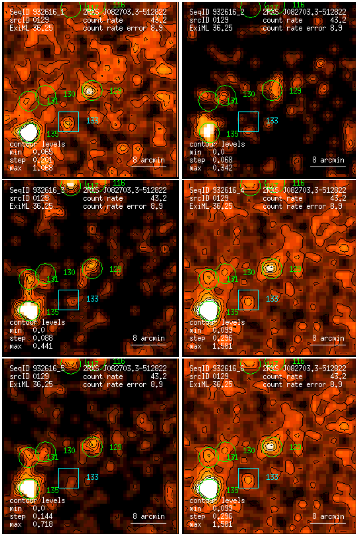
Figure 129: RASS 932616: detection 0129: band rate images, Gaussian filter: (1) PSPC channels 11 – 41, (2) 52 – 90, (3) 91 – 201, (4) 11 – 235, (5) 52 – 201, (6) 11 – 201. Broad band rates in counts/ks. Band rate contour levels in counts/ks/arcmin 2 .
