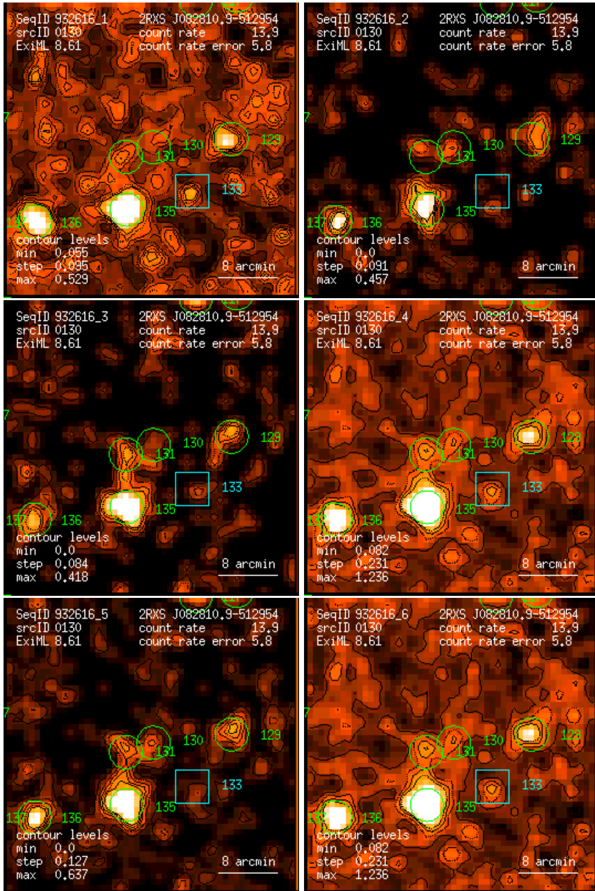
Figure 130: RASS 932616: detection 0130: band rate images, Gaussian filter: (1) PSPC channels 11 – 41, (2) 52 – 90, (3) 91 – 201, (4) 11 – 235, (5) 52 – 201, (6) 11 – 201. Broad band rates in counts/ks. Band rate contour levels in counts/ks/arcmin 2 .
