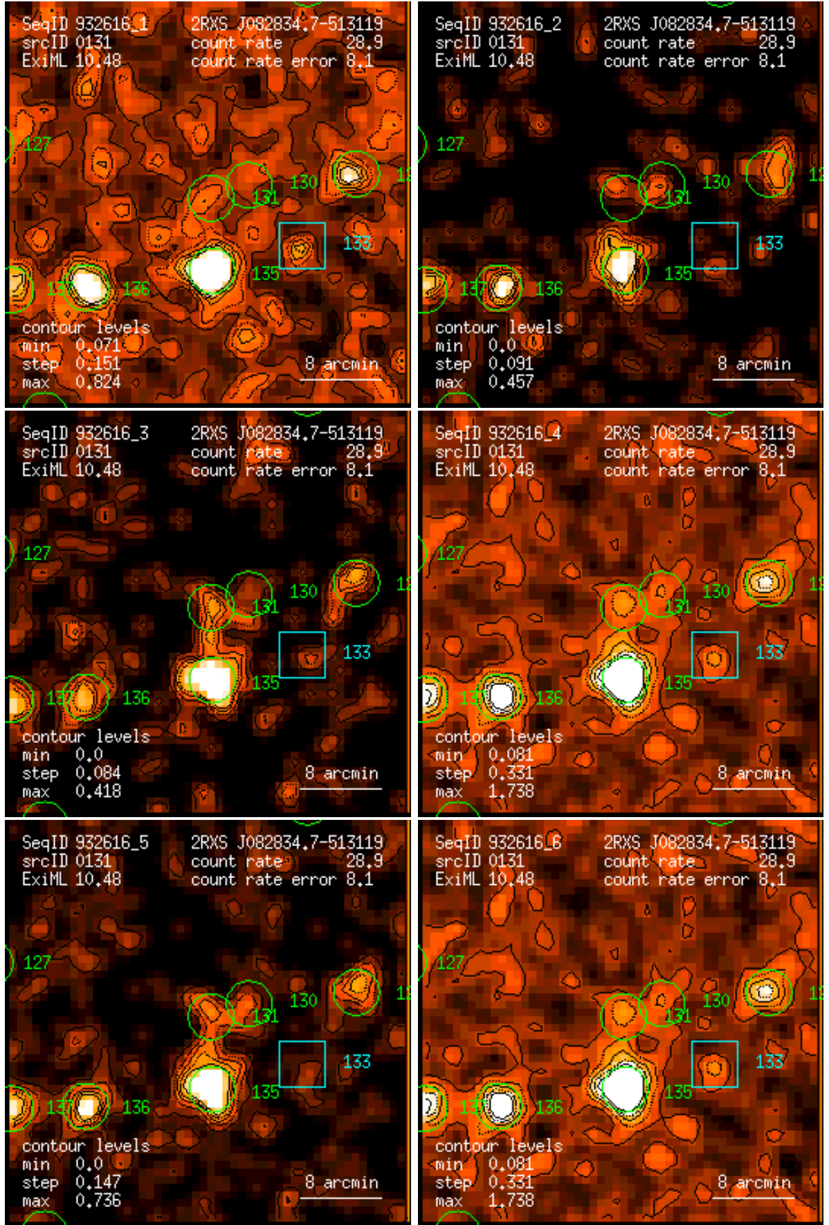
Figure 131: RASS 932616: detection 0131: band rate images, Gaussian filter: (1) PSPC channels 11 – 41, (2) 52 – 90, (3) 91 – 201, (4) 11 – 235, (5) 52 – 201, (6) 11 – 201. Broad band rates in counts/ks. Band rate contour levels in counts/ks/arcmin 2 .
