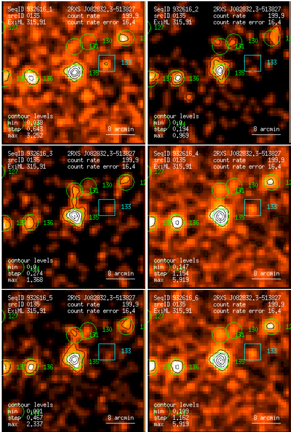
Figure 135: RASS 932616: detection 0135: band rate images, Gaussian filter: (1) PSPC channels 11 – 41, (2) 52 – 90, (3) 91 – 201, (4) 11 – 235, (5) 52 – 201, (6) 11 – 201. Broad band rates in counts/ks. Band rate contour levels in counts/ks/arcmin 2 .
