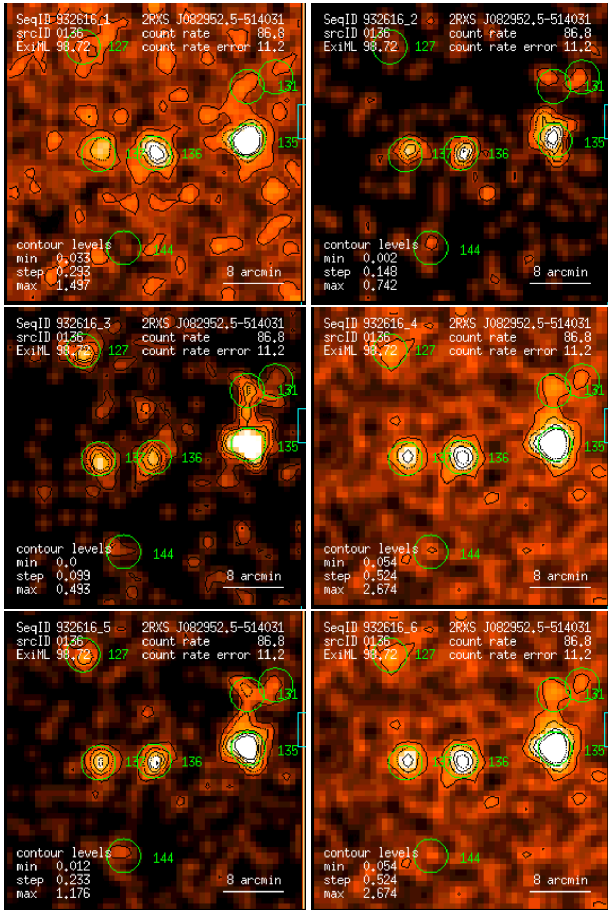
Figure 136: RASS 932616: detection 0136: band rate images, Gaussian filter: (1) PSPC channels 11 – 41, (2) 52 – 90, (3) 91 – 201, (4) 11 – 235, (5) 52 – 201, (6) 11 – 201. Broad band rates in counts/ks. Band rate contour levels in counts/ks/arcmin 2 .
