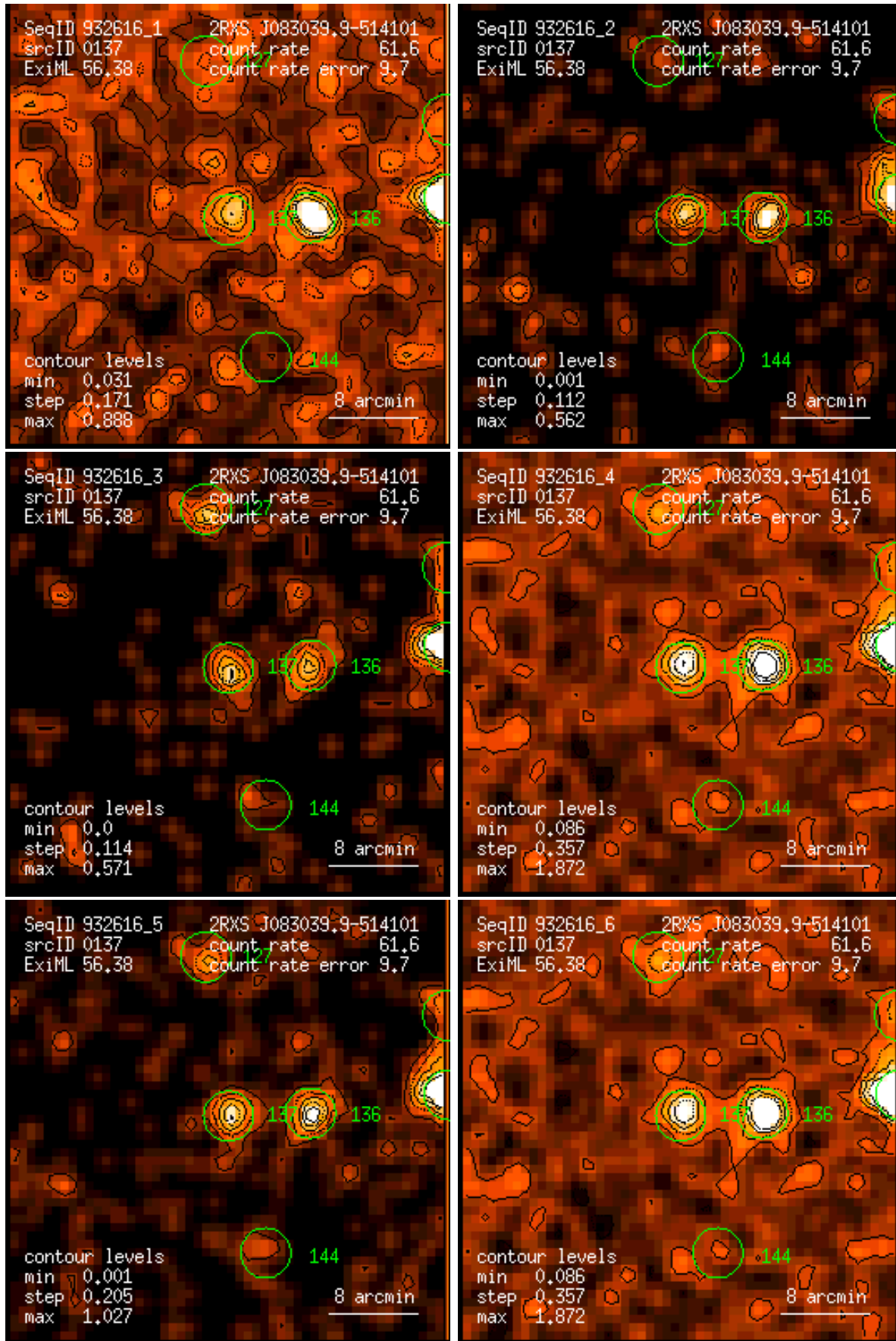
Figure 137: RASS 932616: detection 0137: band rate images, Gaussian filter: (1) PSPC channels 11 – 41, (2) 52 – 90, (3) 91 – 201, (4) 11 – 235, (5) 52 – 201, (6) 11 – 201. Broad band rates in counts/ks. Band rate contour levels in counts/ks/arcmin 2 .
