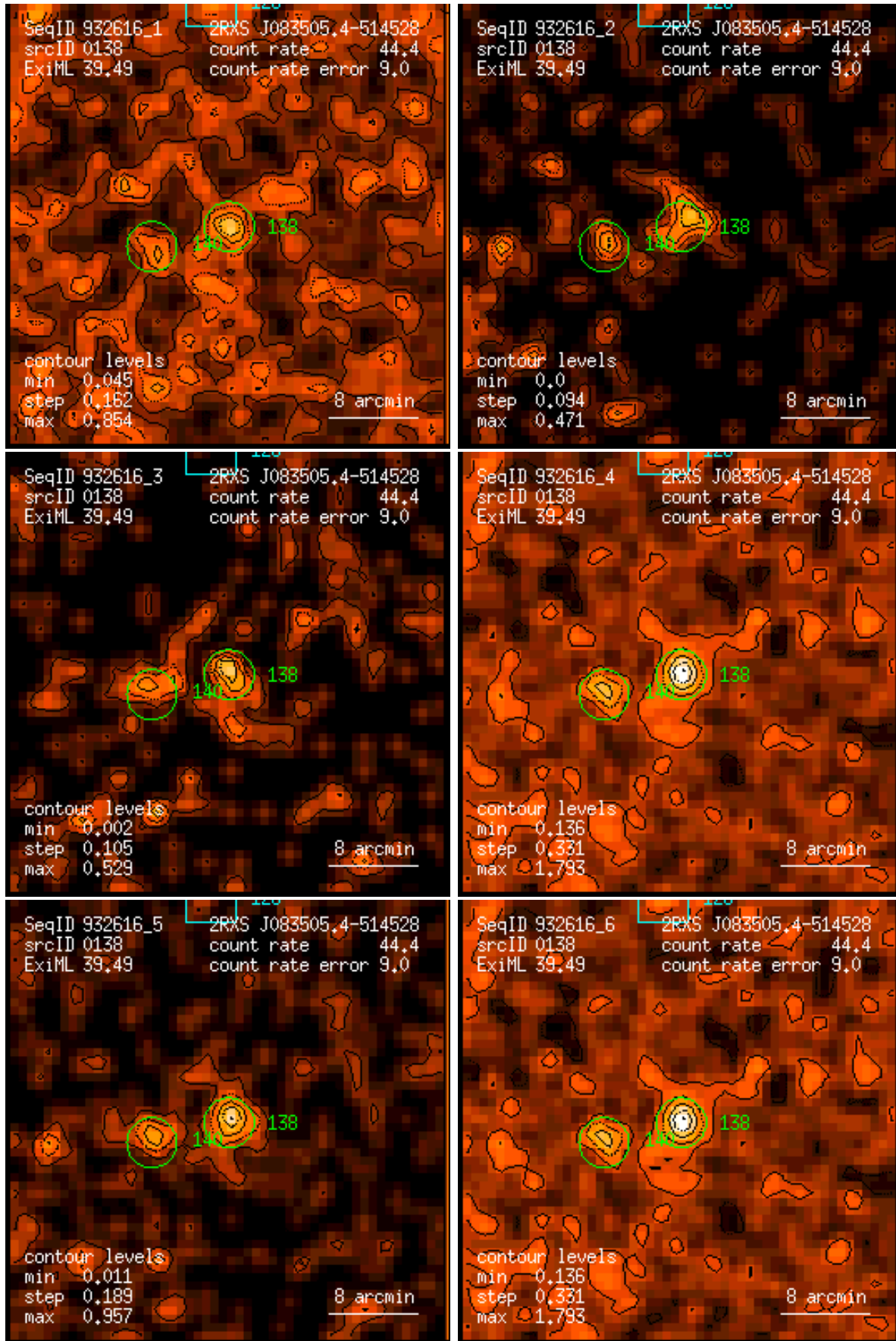
Figure 138: RASS 932616: detection 0138: band rate images, Gaussian filter: (1) PSPC channels 11 – 41, (2) 52 – 90, (3) 91 – 201, (4) 11 – 235, (5) 52 – 201, (6) 11 – 201. Broad band rates in counts/ks. Band rate contour levels in counts/ks/arcmin 2 .
