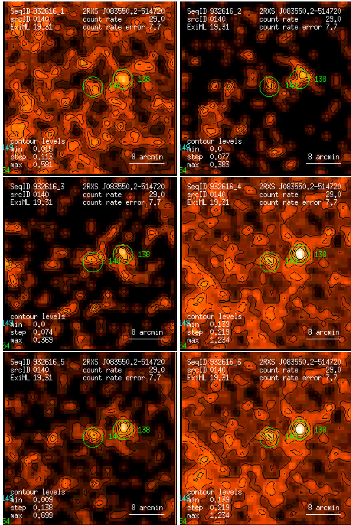
Figure 140: RASS 932616: detection 0140: band rate images, Gaussian filter: (1) PSPC channels 11 – 41, (2) 52 – 90, (3) 91 – 201, (4) 11 – 235, (5) 52 – 201, (6) 11 – 201. Broad band rates in counts/ks. Band rate contour levels in counts/ks/arcmin 2 .
