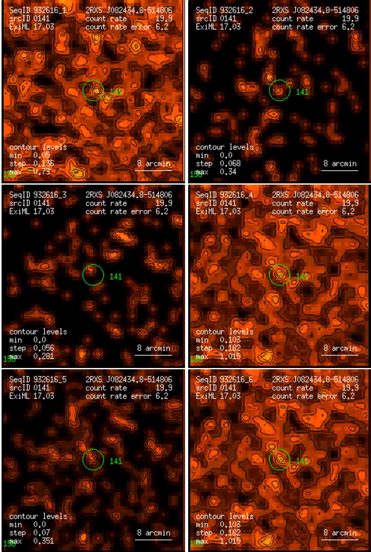
Figure 141: RASS 932616: detection 0141: band rate images, Gaussian filter: (1) PSPC channels 11 – 41, (2) 52 – 90, (3) 91 – 201, (4) 11 – 235, (5) 52 – 201, (6) 11 – 201. Broad band rates in counts/ks. Band rate contour levels in counts/ks/arcmin 2 .
