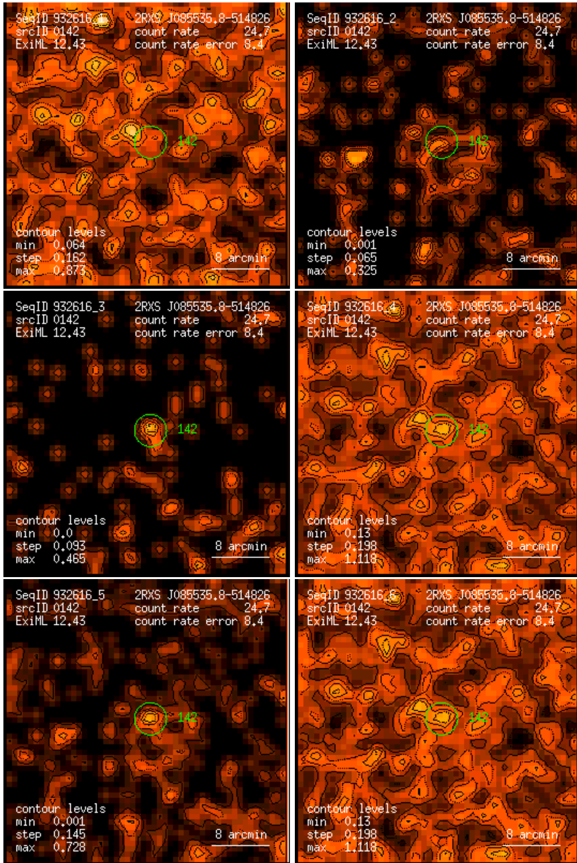
Figure 142: RASS 932616: detection 0142: band rate images, Gaussian filter: (1) PSPC channels 11 – 41, (2) 52 – 90, (3) 91 – 201, (4) 11 – 235, (5) 52 – 201, (6) 11 – 201. Broad band rates in counts/ks. Band rate contour levels in counts/ks/arcmin 2 .
