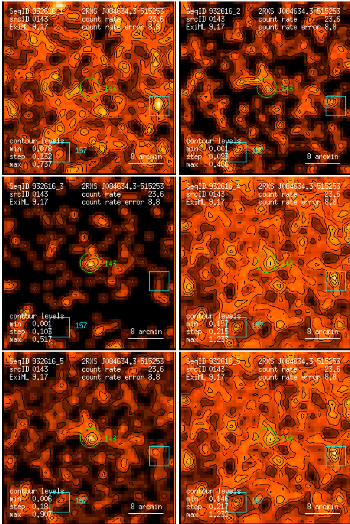
Figure 143: RASS 932616: detection 0143: band rate images, Gaussian filter: (1) PSPC channels 11 – 41, (2) 52 – 90, (3) 91 – 201, (4) 11 – 235, (5) 52 – 201, (6) 11 – 201. Broad band rates in counts/ks. Band rate contour levels in counts/ks/arcmin 2 .
