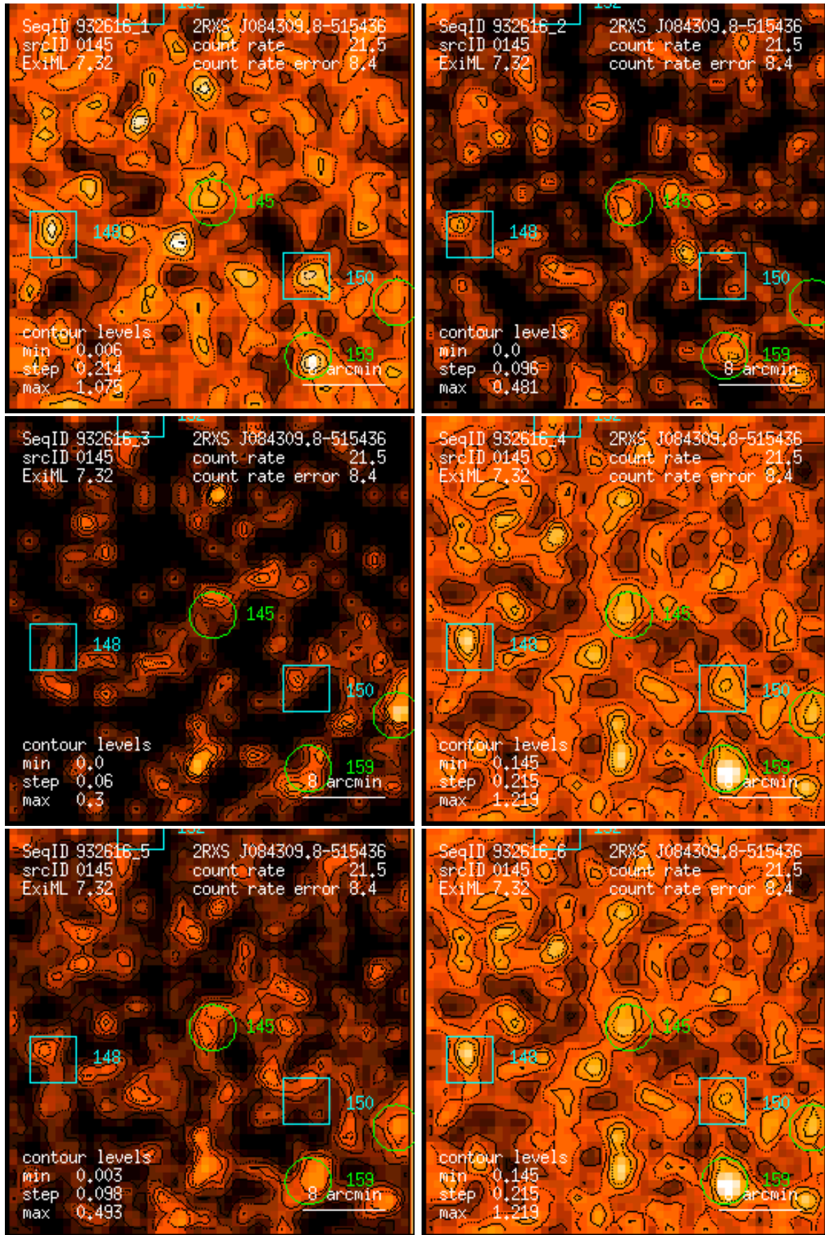
Figure 145: RASS 932616: detection 0145: band rate images, Gaussian filter: (1) PSPC channels 11 – 41, (2) 52 – 90, (3) 91 – 201, (4) 11 – 235, (5) 52 – 201, (6) 11 – 201. Broad band rates in counts/ks. Band rate contour levels in counts/ks/arcmin 2 .
