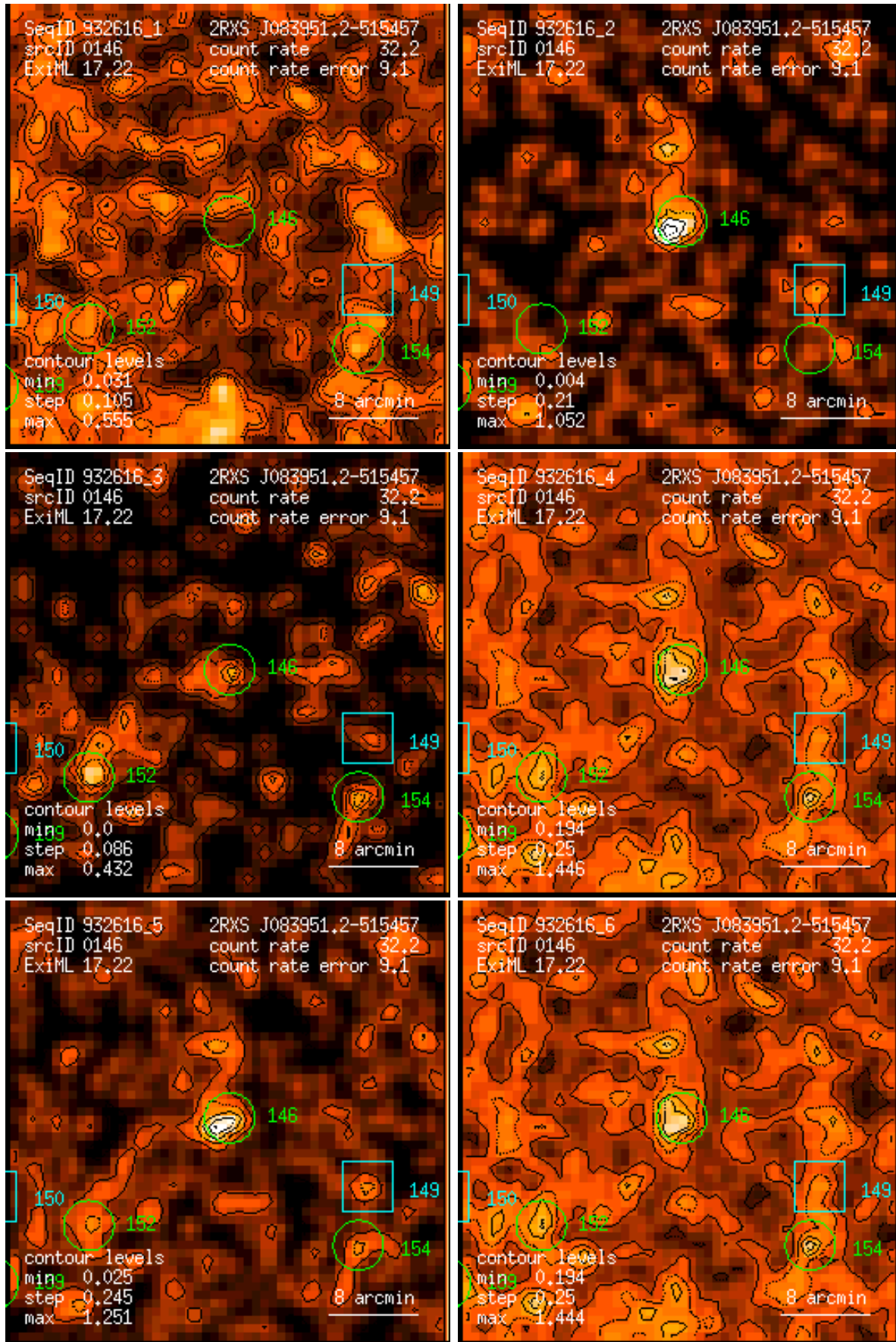
Figure 146: RASS 932616: detection 0146: band rate images, Gaussian filter: (1) PSPC channels 11 – 41, (2) 52 – 90, (3) 91 – 201, (4) 11 – 235, (5) 52 – 201, (6) 11 – 201. Broad band rates in counts/ks. Band rate contour levels in counts/ks/arcmin 2 .
