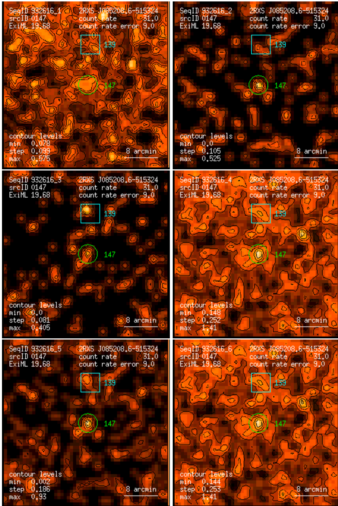
Figure 147: RASS 932616: detection 0147: band rate images, Gaussian filter: (1) PSPC channels 11 – 41, (2) 52 – 90, (3) 91 – 201, (4) 11 – 235, (5) 52 – 201, (6) 11 – 201. Broad band rates in counts/ks. Band rate contour levels in counts/ks/arcmin 2 .
