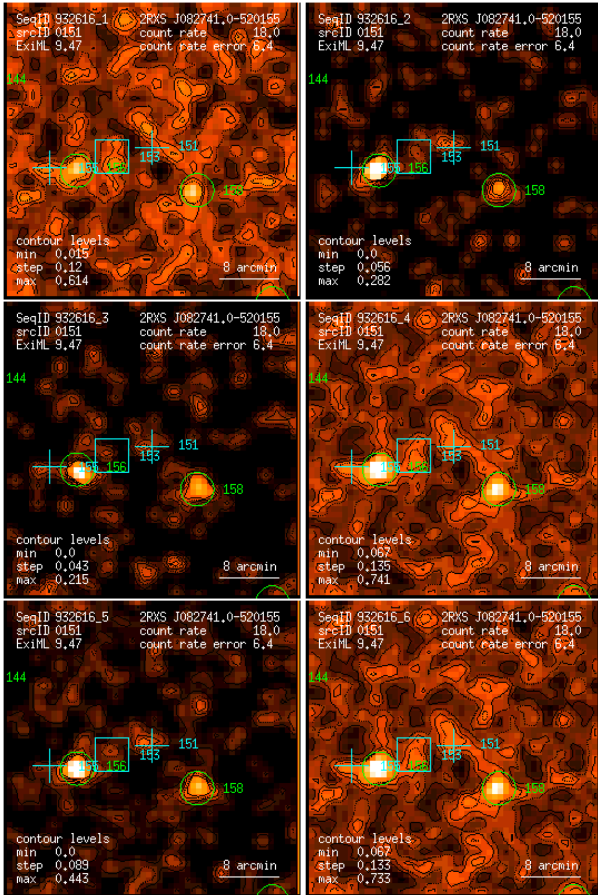
Figure 151: RASS 932616: detection 0151: band rate images, Gaussian filter: (1) PSPC channels 11 – 41, (2) 52 – 90, (3) 91 – 201, (4) 11 – 235, (5) 52 – 201, (6) 11 – 201. Broad band rates in counts/ks. Band rate contour levels in counts/ks/arcmin 2 .
