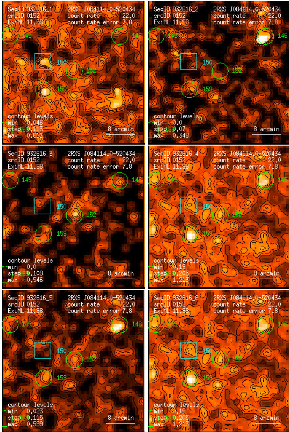
Figure 152: RASS 932616: detection 0152: band rate images, Gaussian filter: (1) PSPC channels 11 – 41, (2) 52 – 90, (3) 91 – 201, (4) 11 – 235, (5) 52 – 201, (6) 11 – 201. Broad band rates in counts/ks. Band rate contour levels in counts/ks/arcmin 2 .
