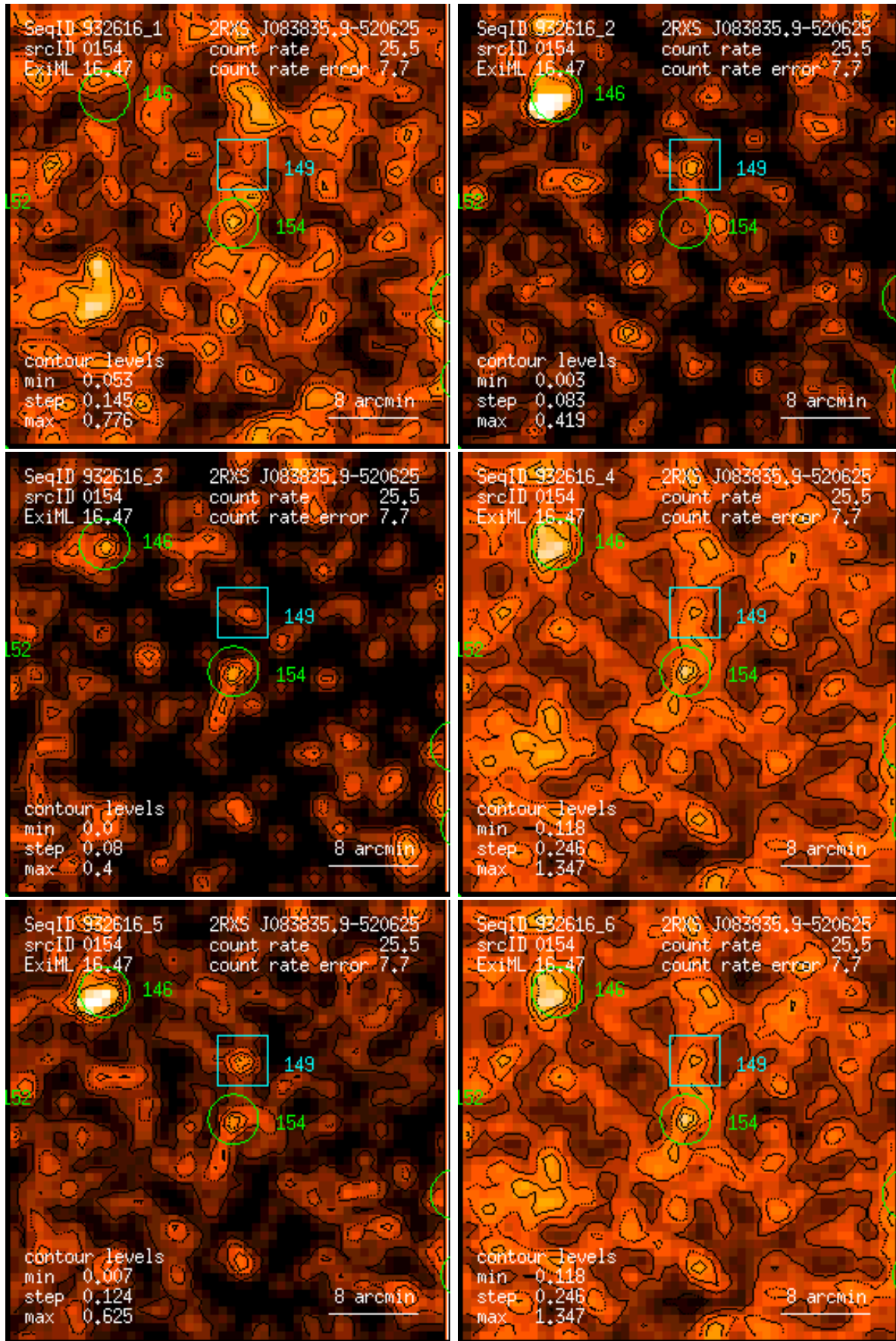
Figure 154: RASS 932616: detection 0154: band rate images, Gaussian filter: (1) PSPC channels 11 – 41, (2) 52 – 90, (3) 91 – 201, (4) 11 – 235, (5) 52 – 201, (6) 11 – 201. Broad band rates in counts/ks. Band rate contour levels in counts/ks/arcmin 2 .
