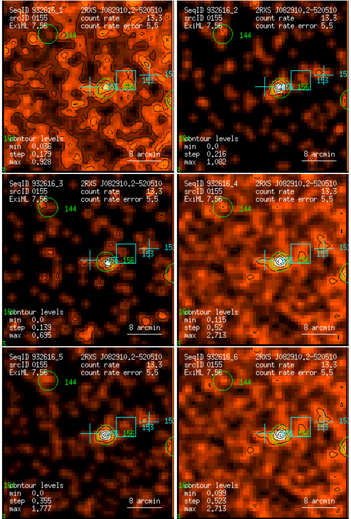
Figure 155: RASS 932616: detection 0155: band rate images, Gaussian filter: (1) PSPC channels 11 – 41, (2) 52 – 90, (3) 91 – 201, (4) 11 – 235, (5) 52 – 201, (6) 11 – 201. Broad band rates in counts/ks. Band rate contour levels in counts/ks/arcmin 2 .
