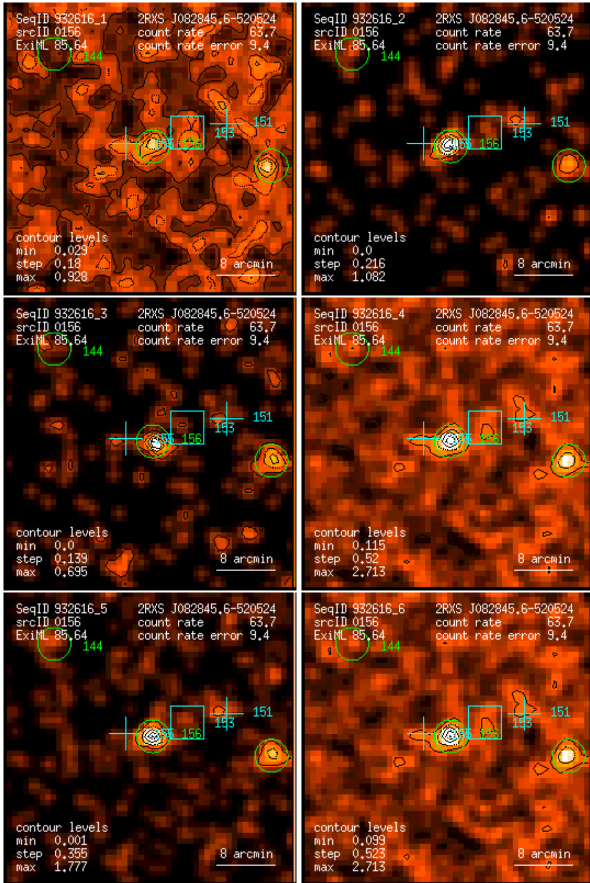
Figure 156: RASS 932616: detection 0156: band rate images, Gaussian filter: (1) PSPC channels 11 – 41, (2) 52 – 90, (3) 91 – 201, (4) 11 – 235, (5) 52 – 201, (6) 11 – 201. Broad band rates in counts/ks. Band rate contour levels in counts/ks/arcmin 2 .
