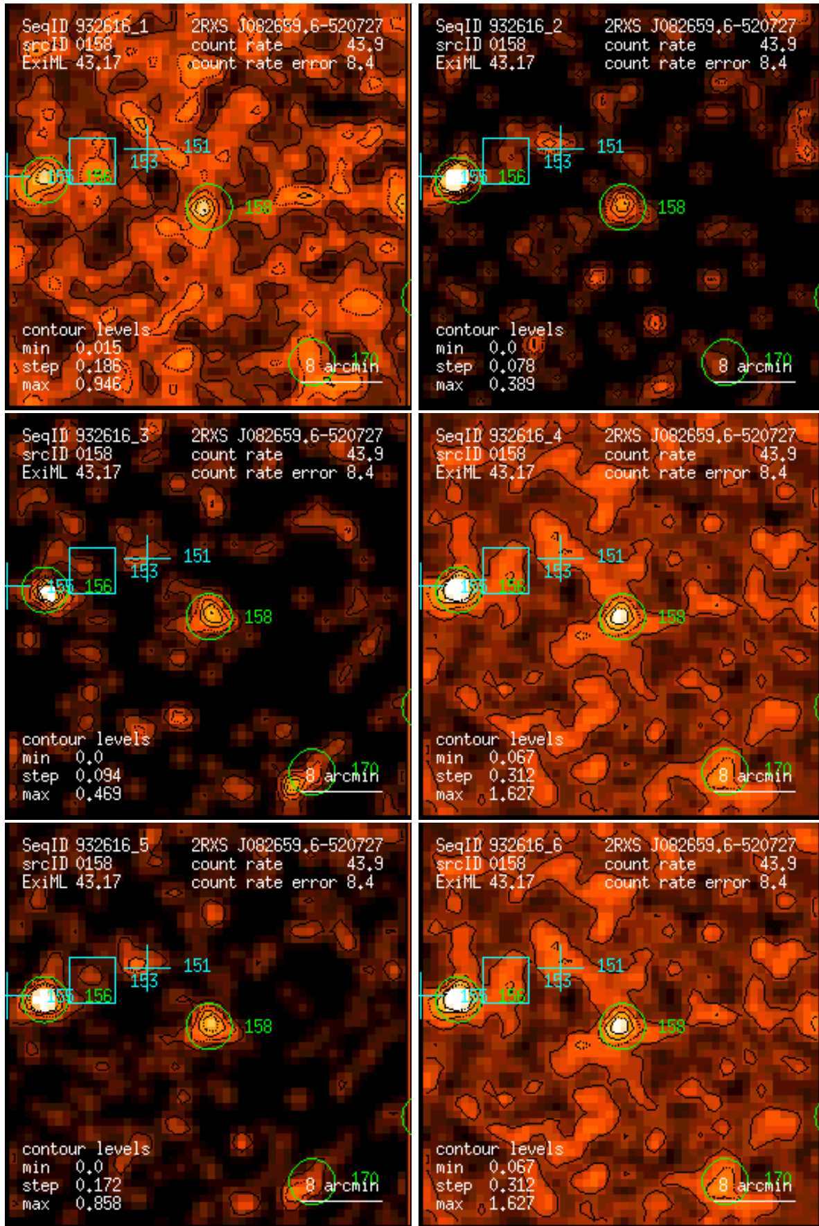
Figure 158: RASS 932616: detection 0158: band rate images, Gaussian filter: (1) PSPC channels 11 – 41, (2) 52 – 90, (3) 91 – 201, (4) 11 – 235, (5) 52 – 201, (6) 11 – 201. Broad band rates in counts/ks. Band rate contour levels in counts/ks/arcmin 2 .
