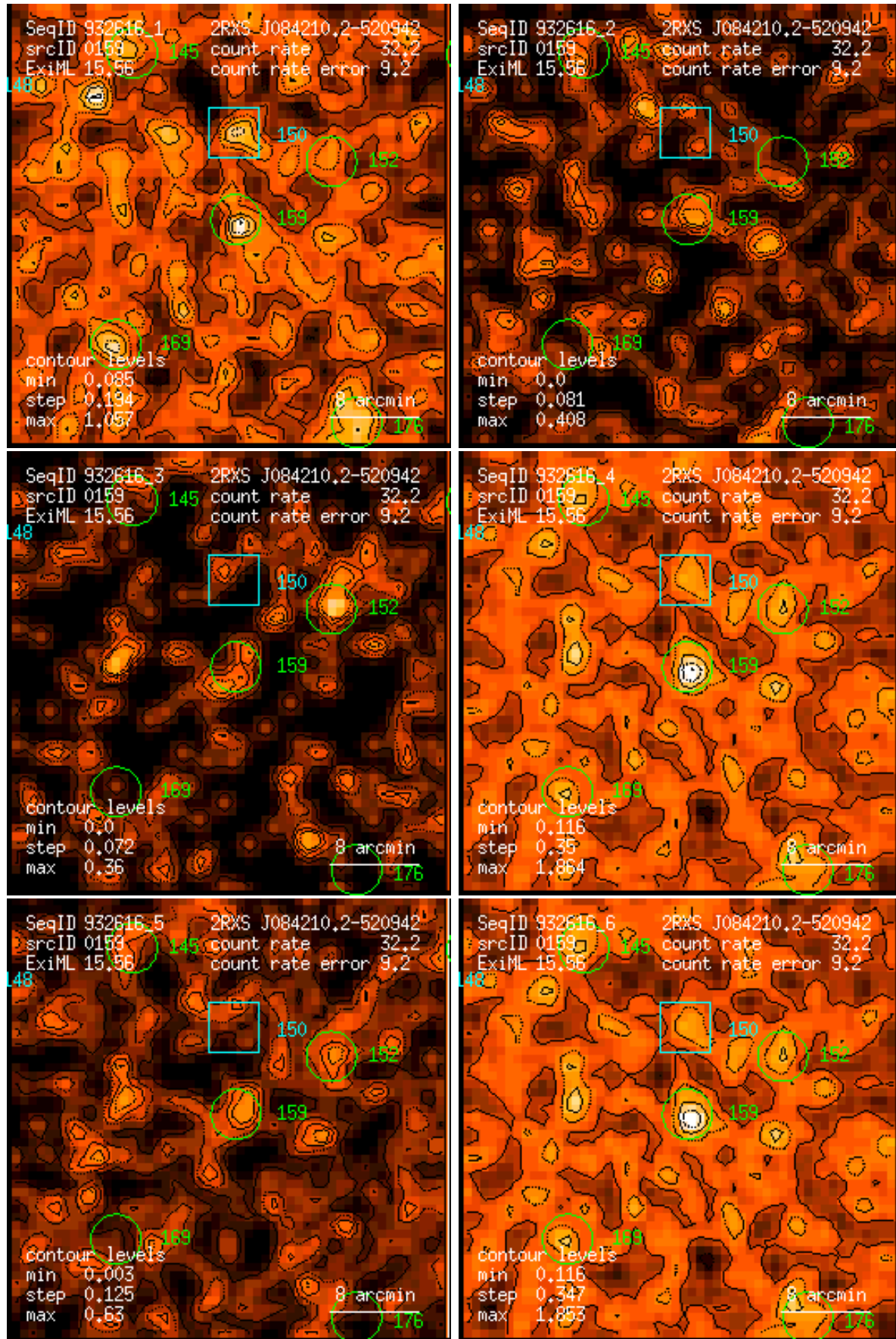
Figure 159: RASS 932616: detection 0159: band rate images, Gaussian filter: (1) PSPC channels 11 – 41, (2) 52 – 90, (3) 91 – 201, (4) 11 – 235, (5) 52 – 201, (6) 11 – 201. Broad band rates in counts/ks. Band rate contour levels in counts/ks/arcmin 2 .
