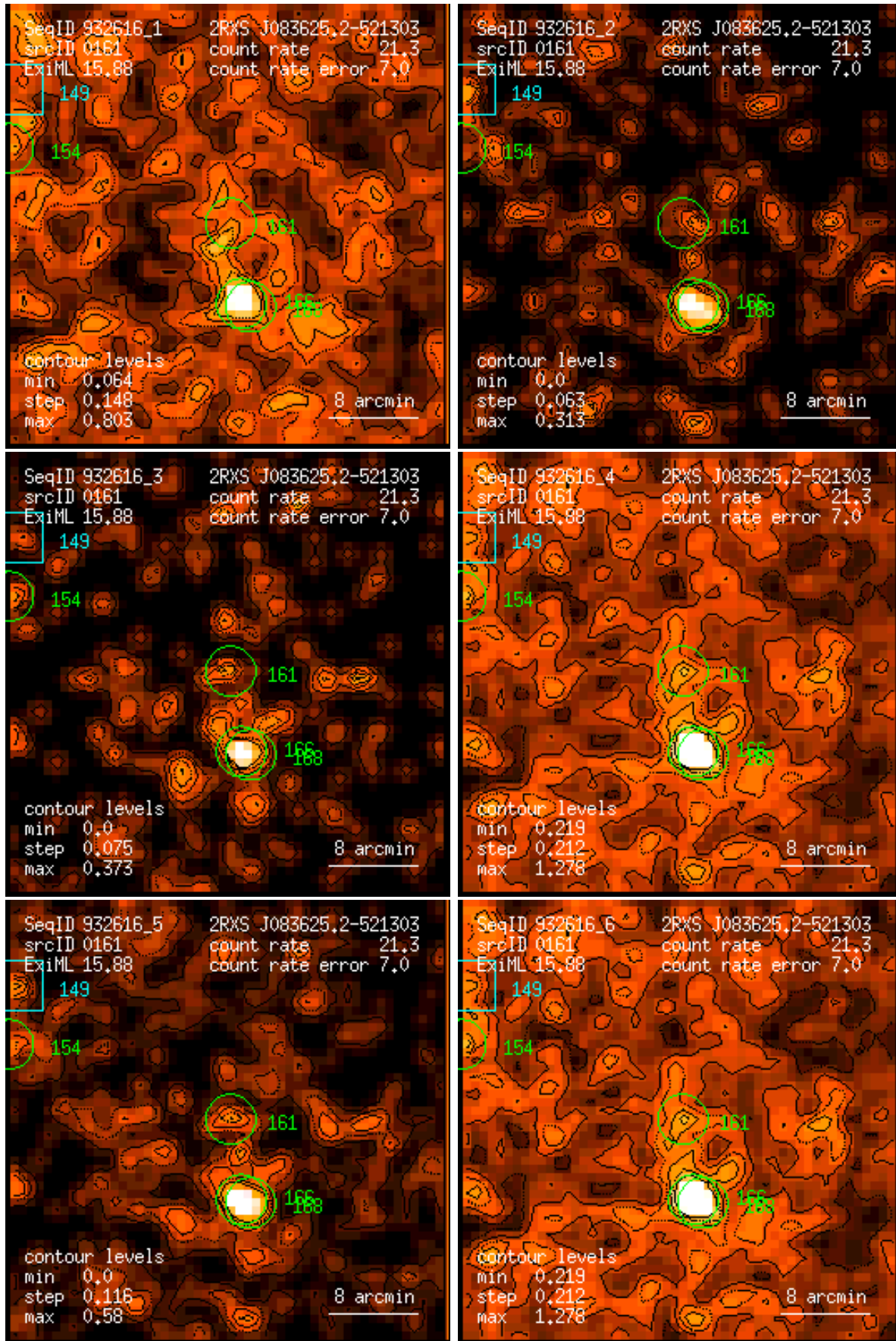
Figure 161: RASS 932616: detection 0161: band rate images, Gaussian filter: (1) PSPC channels 11 – 41, (2) 52 – 90, (3) 91 – 201, (4) 11 – 235, (5) 52 – 201, (6) 11 – 201. Broad band rates in counts/ks. Band rate contour levels in counts/ks/arcmin 2 .
