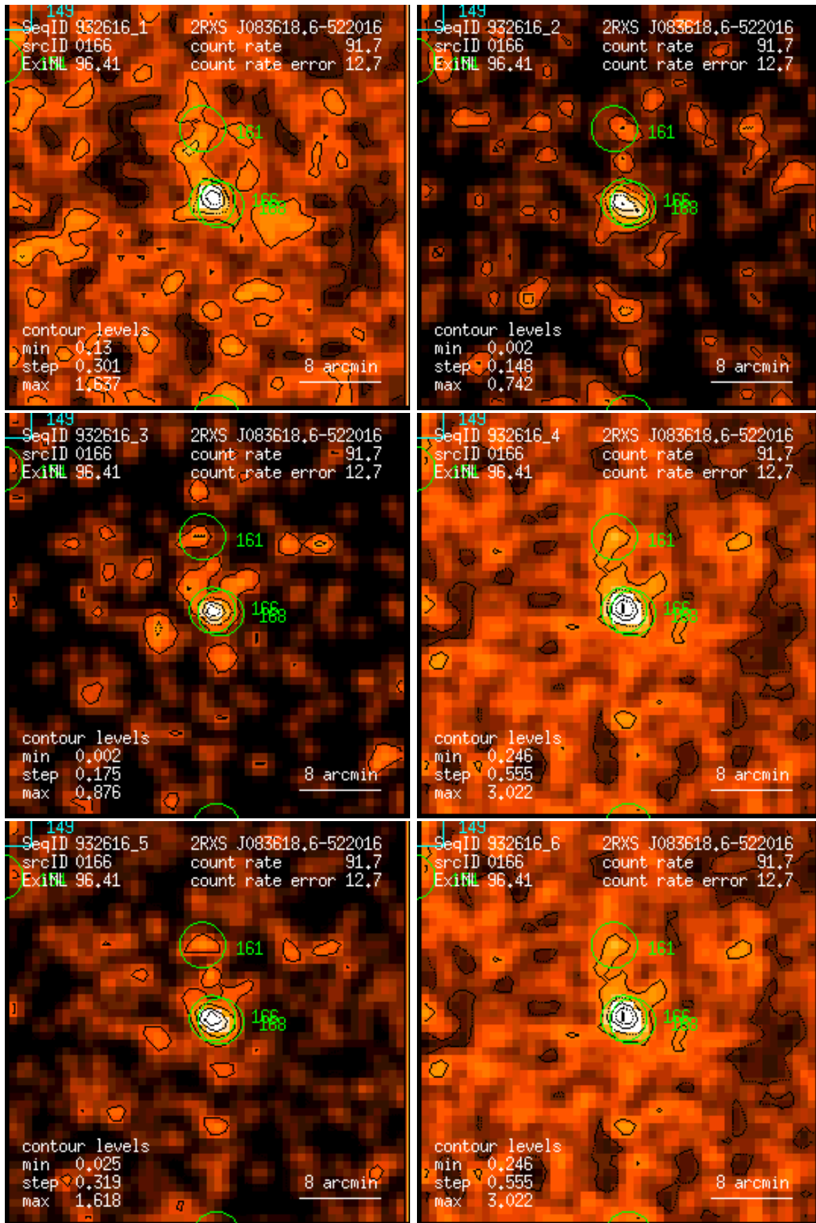
Figure 166: RASS 932616: detection 0166: band rate images, Gaussian filter: (1) PSPC channels 11 – 41, (2) 52 – 90, (3) 91 – 201, (4) 11 – 235, (5) 52 – 201, (6) 11 – 201. Broad band rates in counts/ks. Band rate contour levels in counts/ks/arcmin 2 .
