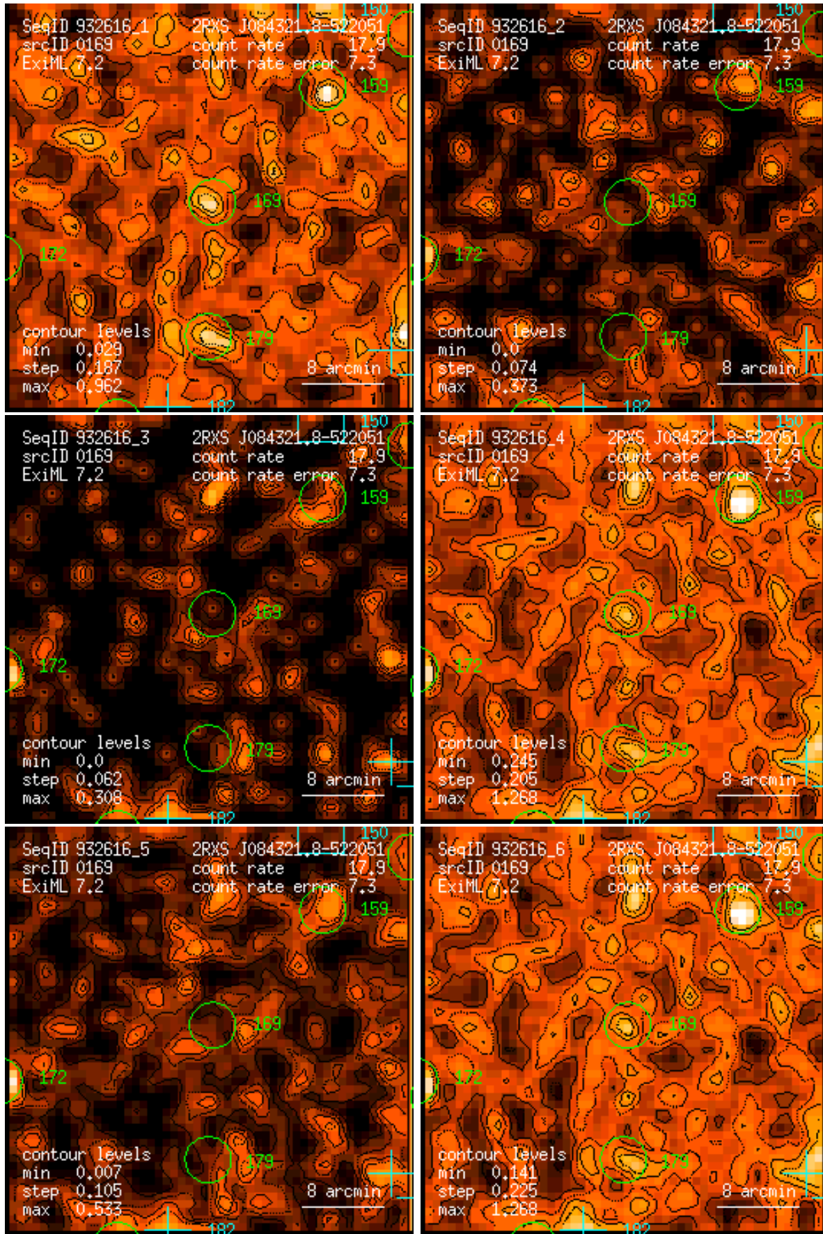
Figure 169: RASS 932616: detection 0169: band rate images, Gaussian filter: (1) PSPC channels 11 – 41, (2) 52 – 90, (3) 91 – 201, (4) 11 – 235, (5) 52 – 201, (6) 11 – 201. Broad band rates in counts/ks. Band rate contour levels in counts/ks/arcmin 2 .
