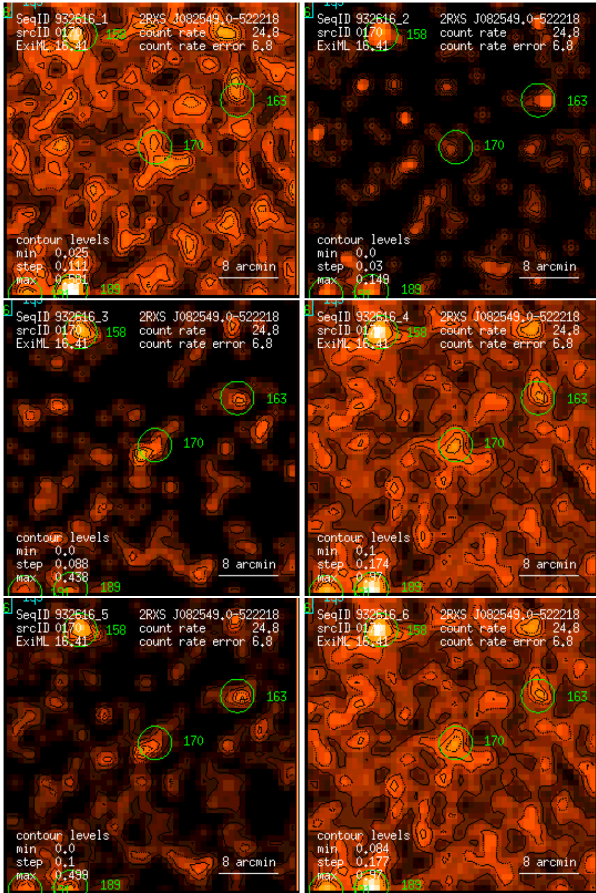
Figure 170: RASS 932616: detection 0170: band rate images, Gaussian filter: (1) PSPC channels 11 – 41, (2) 52 – 90, (3) 91 – 201, (4) 11 – 235, (5) 52 – 201, (6) 11 – 201. Broad band rates in counts/ks. Band rate contour levels in counts/ks/arcmin 2 .
