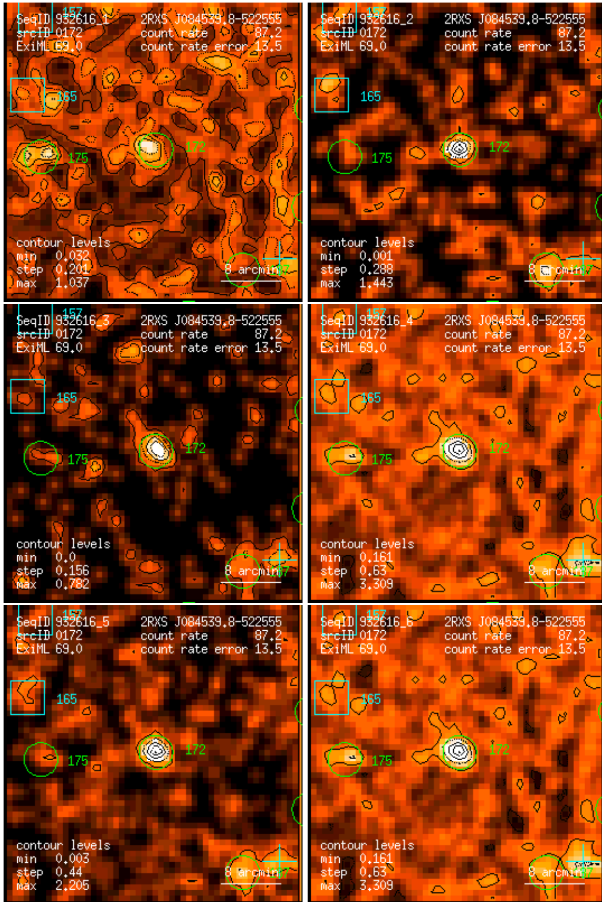
Figure 172: RASS 932616: detection 0172: band rate images, Gaussian filter: (1) PSPC channels 11 – 41, (2) 52 – 90, (3) 91 – 201, (4) 11 – 235, (5) 52 – 201, (6) 11 – 201. Broad band rates in counts/ks. Band rate contour levels in counts/ks/arcmin 2 .
