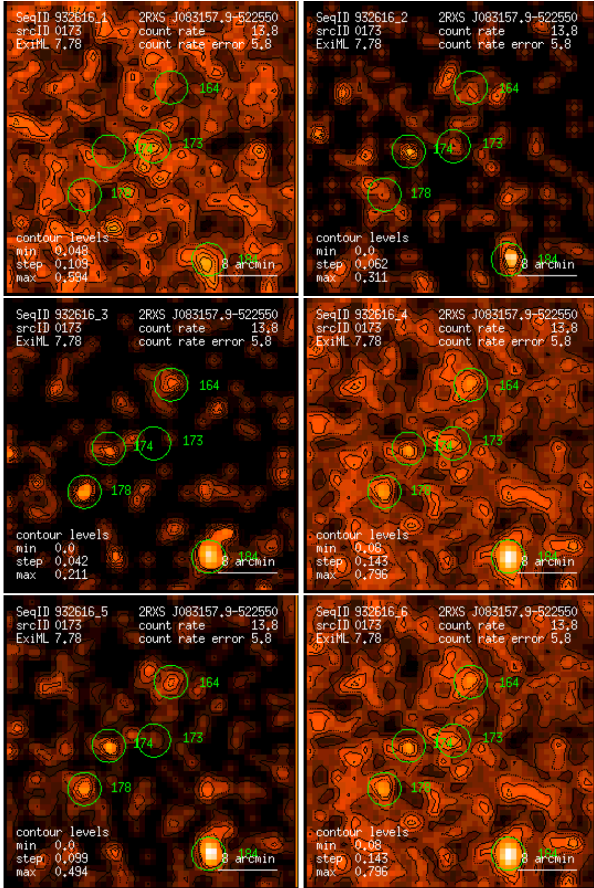
Figure 173: RASS 932616: detection 0173: band rate images, Gaussian filter: (1) PSPC channels 11 – 41, (2) 52 – 90, (3) 91 – 201, (4) 11 – 235, (5) 52 – 201, (6) 11 – 201. Broad band rates in counts/ks. Band rate contour levels in counts/ks/arcmin 2 .
