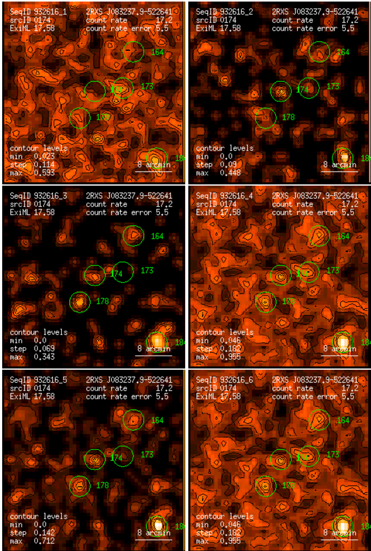
Figure 174: RASS 932616: detection 0174: band rate images, Gaussian filter: (1) PSPC channels 11 – 41, (2) 52 – 90, (3) 91 – 201, (4) 11 – 235, (5) 52 – 201, (6) 11 – 201. Broad band rates in counts/ks. Band rate contour levels in counts/ks/arcmin 2 .
