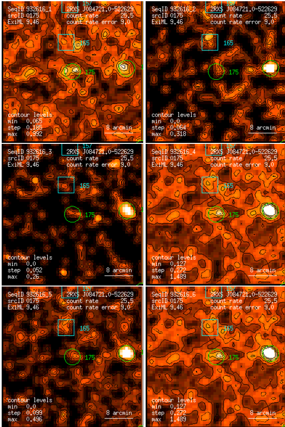
Figure 175: RASS 932616: detection 0175: band rate images, Gaussian filter: (1) PSPC channels 11 – 41, (2) 52 – 90, (3) 91 – 201, (4) 11 – 235, (5) 52 – 201, (6) 11 – 201. Broad band rates in counts/ks. Band rate contour levels in counts/ks/arcmin 2 .
