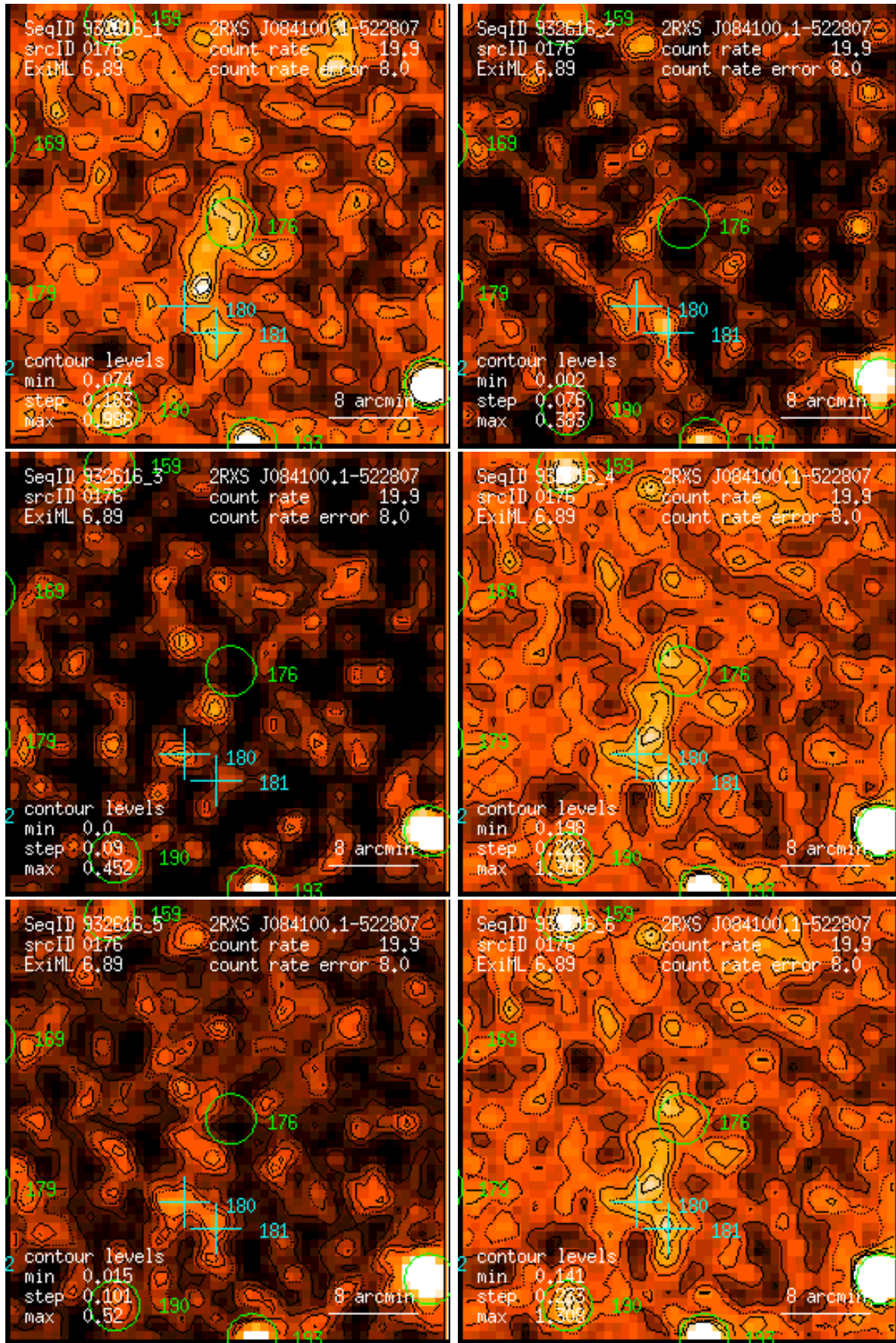
Figure 176: RASS 932616: detection 0176: band rate images, Gaussian filter: (1) PSPC channels 11 – 41, (2) 52 – 90, (3) 91 – 201, (4) 11 – 235, (5) 52 – 201, (6) 11 – 201. Broad band rates in counts/ks. Band rate contour levels in counts/ks/arcmin 2 .
