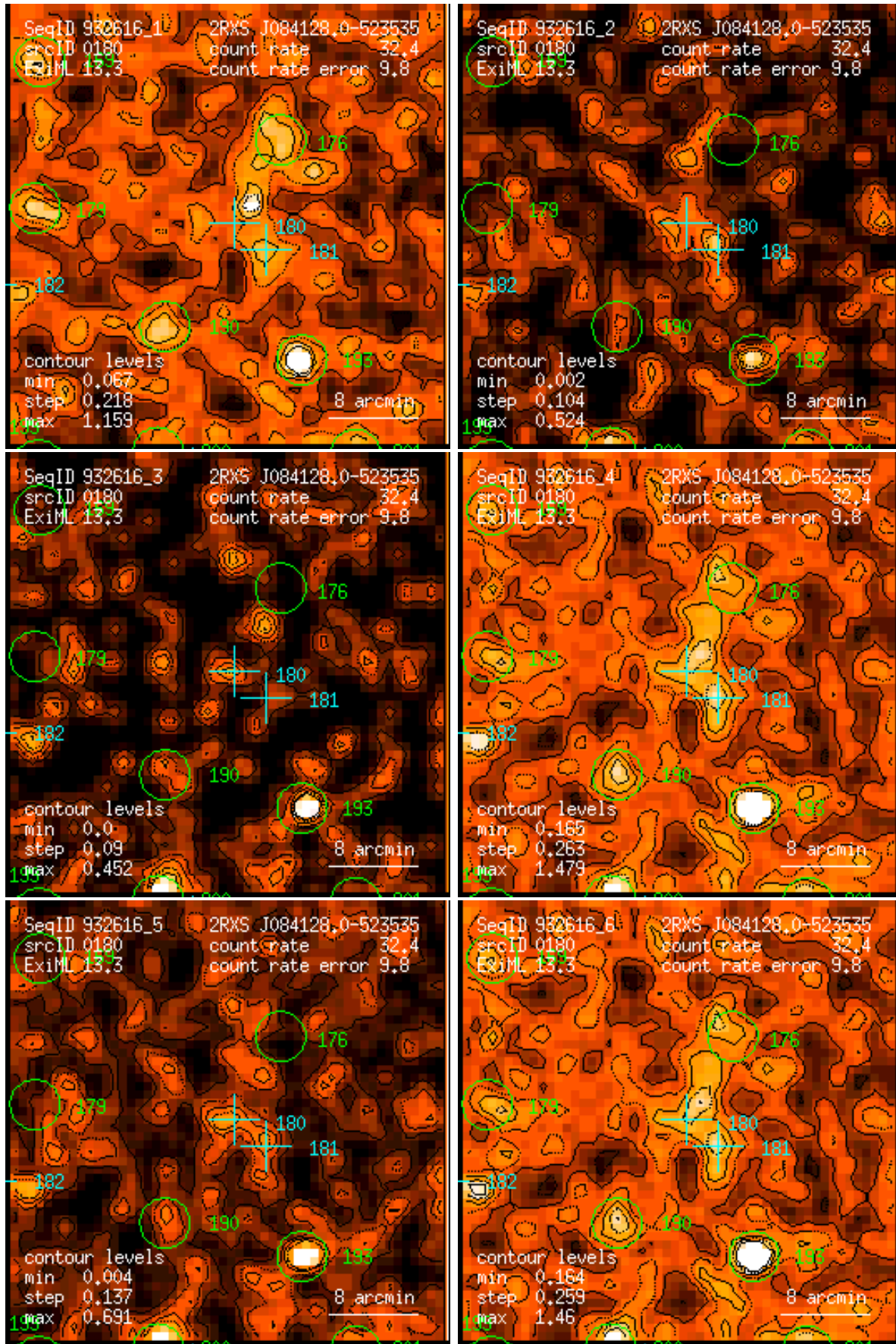
Figure 180: RASS 932616: detection 0180: band rate images, Gaussian filter: (1) PSPC channels 11 – 41, (2) 52 – 90, (3) 91 – 201, (4) 11 – 235, (5) 52 – 201, (6) 11 – 201. Broad band rates in counts/ks. Band rate contour levels in counts/ks/arcmin 2 .
