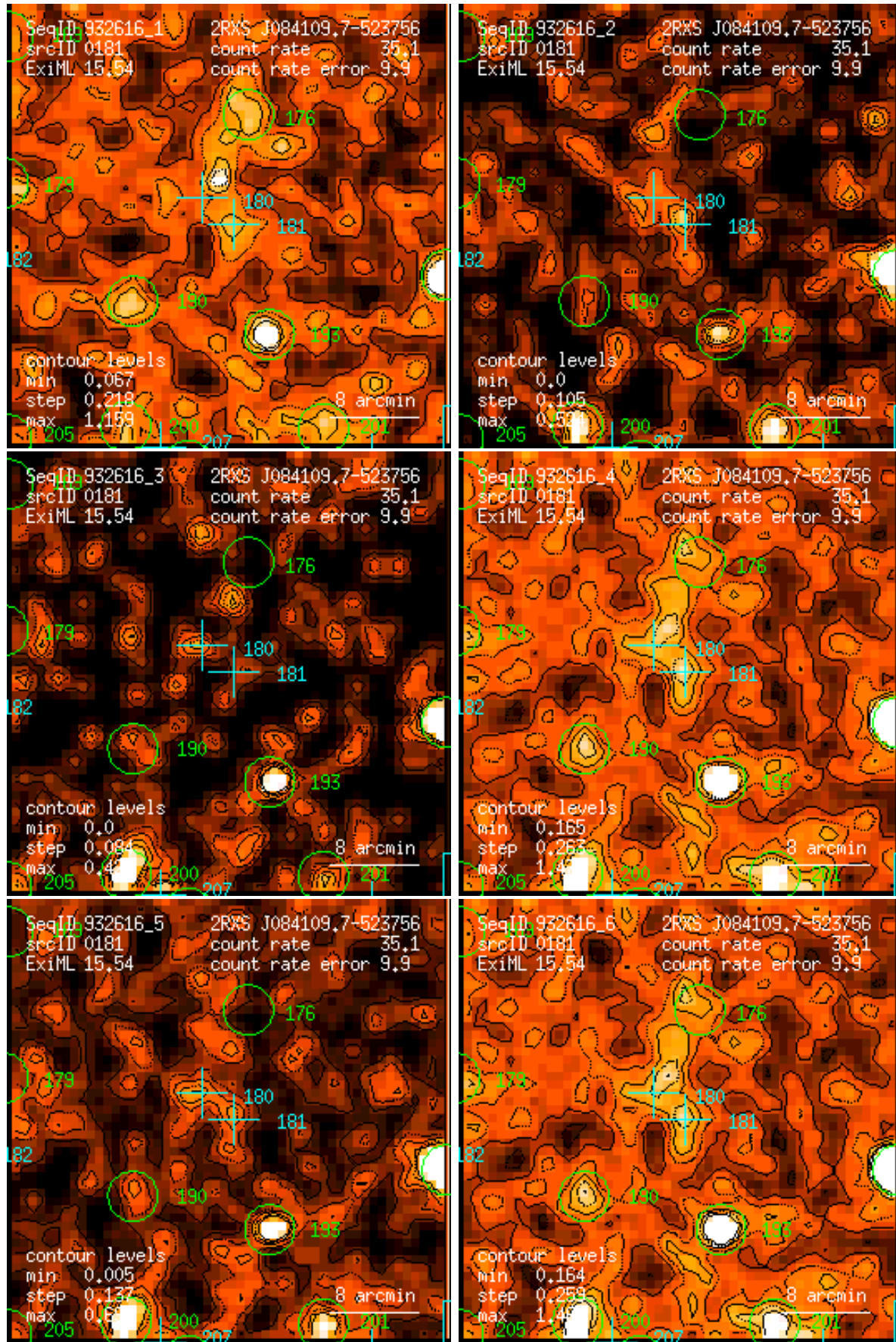
Figure 181: RASS 932616: detection 0181: band rate images, Gaussian filter: (1) PSPC channels 11 – 41, (2) 52 – 90, (3) 91 – 201, (4) 11 – 235, (5) 52 – 201, (6) 11 – 201. Broad band rates in counts/ks. Band rate contour levels in counts/ks/arcmin 2 .
