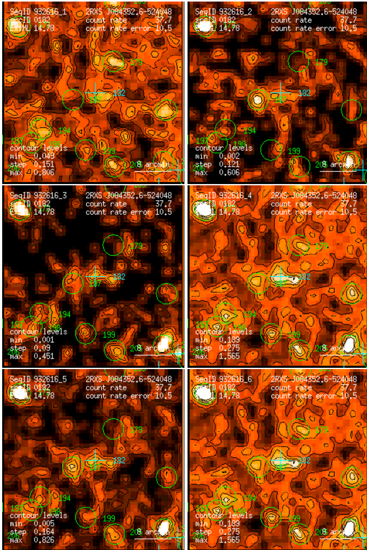
Figure 182: RASS 932616: detection 0182: band rate images, Gaussian filter: (1) PSPC channels 11 – 41, (2) 52 – 90, (3) 91 – 201, (4) 11 – 235, (5) 52 – 201, (6) 11 – 201. Broad band rates in counts/ks. Band rate contour levels in counts/ks/arcmin 2 .
