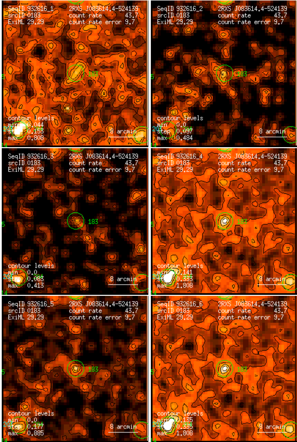
Figure 183: RASS 932616: detection 0183: band rate images, Gaussian filter: (1) PSPC channels 11 – 41, (2) 52 – 90, (3) 91 – 201, (4) 11 – 235, (5) 52 – 201, (6) 11 – 201. Broad band rates in counts/ks. Band rate contour levels in counts/ks/arcmin 2 .
