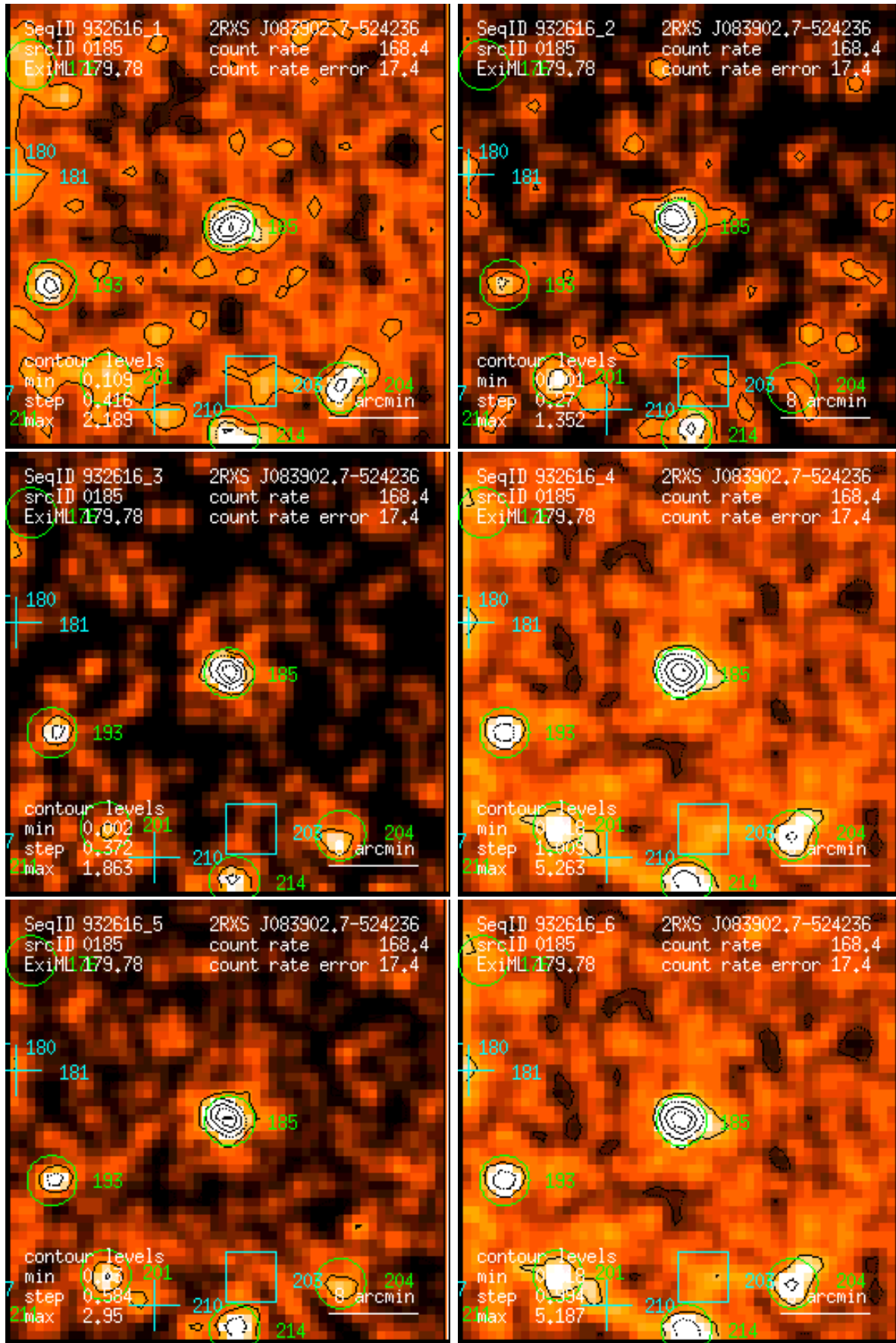
Figure 185: RASS 932616: detection 0185: band rate images, Gaussian filter: (1) PSPC channels 11 – 41, (2) 52 – 90, (3) 91 – 201, (4) 11 – 235, (5) 52 – 201, (6) 11 – 201. Broad band rates in counts/ks. Band rate contour levels in counts/ks/arcmin 2 .
