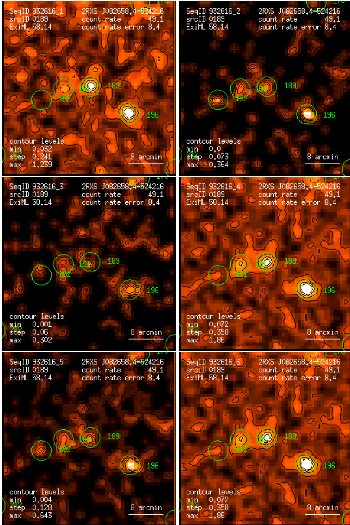
Figure 189: RASS 932616: detection 0189: band rate images, Gaussian filter: (1) PSPC channels 11 – 41, (2) 52 – 90, (3) 91 – 201, (4) 11 – 235, (5) 52 – 201, (6) 11 – 201. Broad band rates in counts/ks. Band rate contour levels in counts/ks/arcmin 2 .
