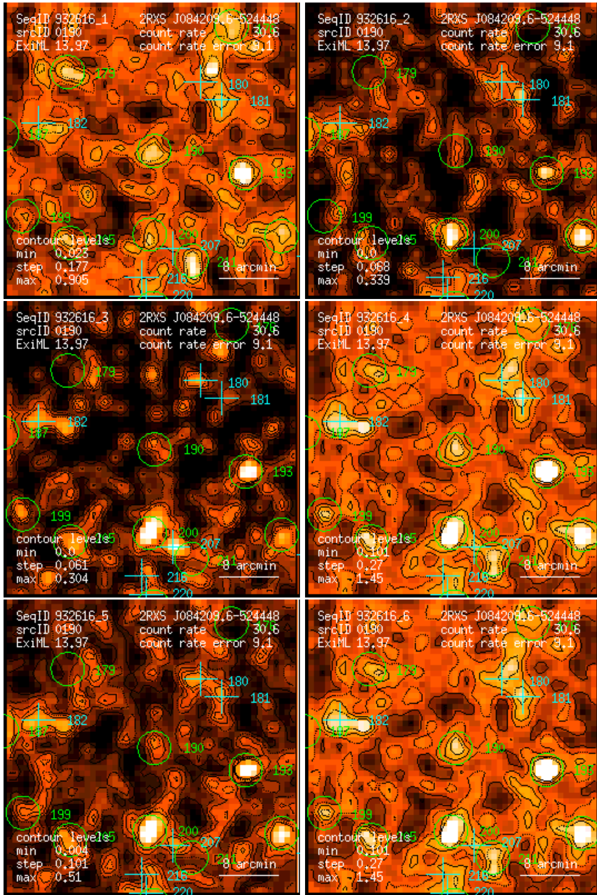
Figure 190: RASS 932616: detection 0190: band rate images, Gaussian filter: (1) PSPC channels 11 – 41, (2) 52 – 90, (3) 91 – 201, (4) 11 – 235, (5) 52 – 201, (6) 11 – 201. Broad band rates in counts/ks. Band rate contour levels in counts/ks/arcmin 2 .
