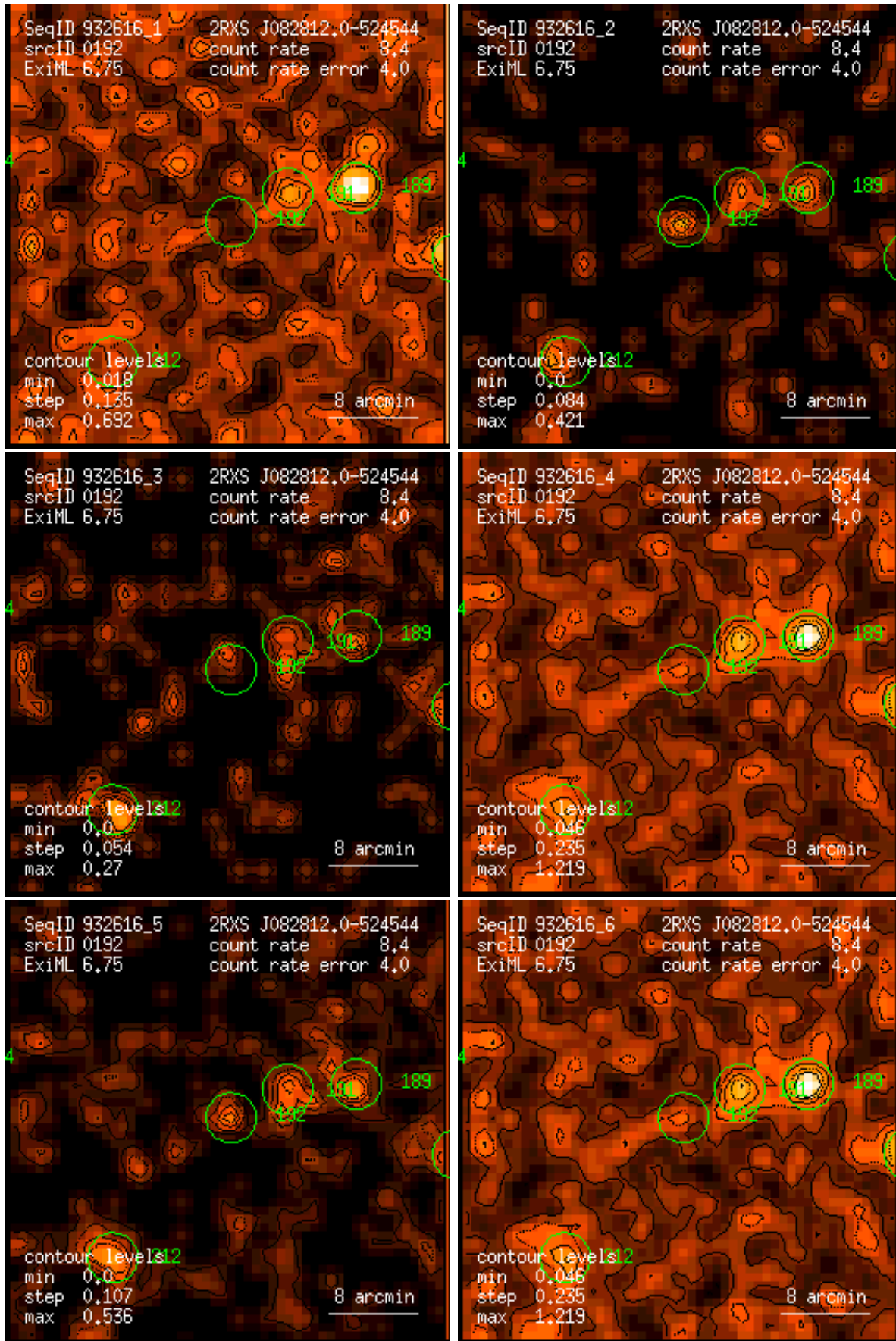
Figure 192: RASS 932616: detection 0192: band rate images, Gaussian filter: (1) PSPC channels 11 – 41, (2) 52 – 90, (3) 91 – 201, (4) 11 – 235, (5) 52 – 201, (6) 11 – 201. Broad band rates in counts/ks. Band rate contour levels in counts/ks/arcmin 2 .
